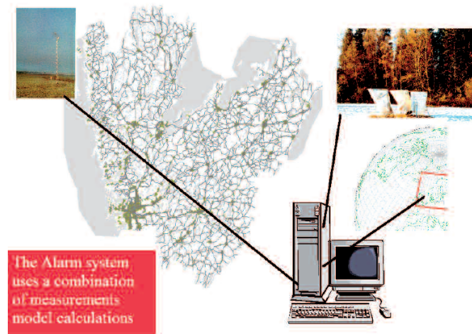
Figure 1. The ALARM-system area located in southwest Sweden. Measurements are collected once per hour and regional prognosis once every 6 th hour. The area size is around 200 x 250 km.
