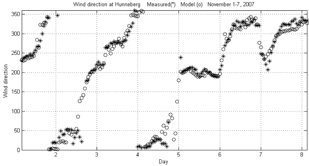
Figure 2. Measured (sodar (*)) and simulated (o) wind directions at site Hunneberg at 175 m.
