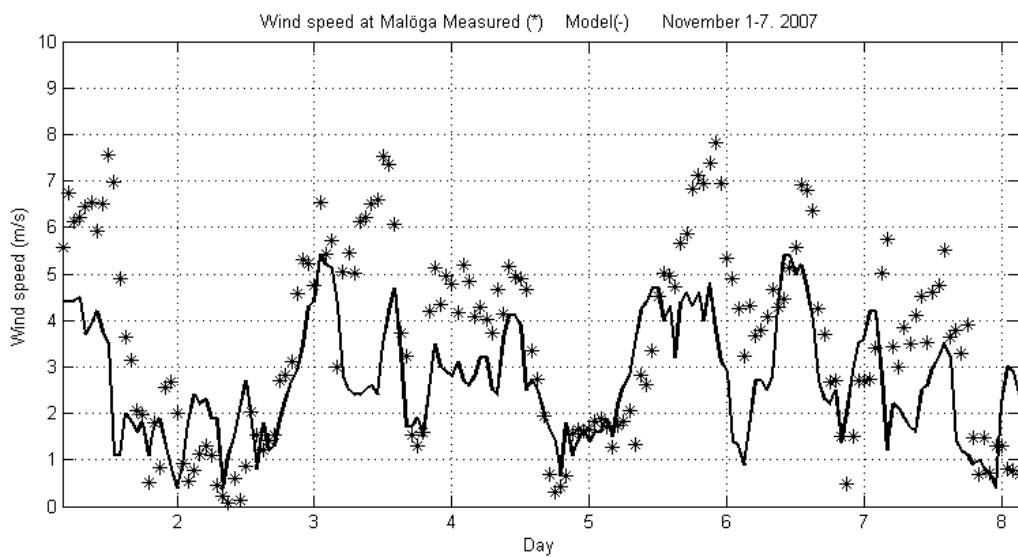
Figure 5. Measured (tower (*)) and simulated (-) wind speed at site Malöga at 10 m.
