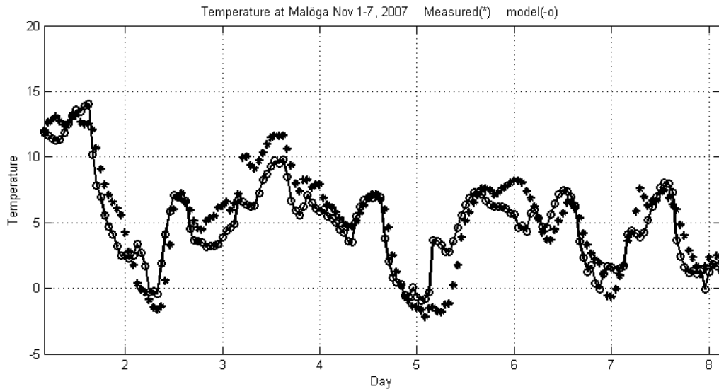
Figure 6. Measured (tower (*)) and simulated (-o-) temperature at site Malöga at 2 m.
