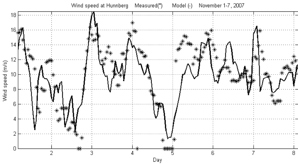
Figure 3. Measured (sodar (*)) and simulated (-) wind speed at site Hunneberg at 175 m.
