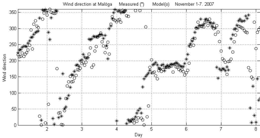
Figure 4. Measured (tower (*)) and simulated (o) wind speed at site Malöga at 10 m.
