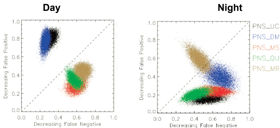
Figure 1. Comparisons of Bootstrap-Resampled User-Oriented Measure of Effectiveness (MOE) Values for Urban T&D Model Predictions of the 17 Daytime (Left) and 12 Nighttime (Right) Releases of JU03 Within the CBD Using the PNS MET Input Option. The models represented are HPAC/Urban Canopy (UC), HPAC/UDM (DM), HPAC/MSS (MS), QUIC-URB/QUIC-PLUME (QU), and MESO/RUSTIC (MR). [MOE values nearer to the “perfect” value of (1,1) represent improved predictions; values “above” the diagonal line correspond to under-predictions, whereas values “below” the diagonal line correspond to over-predictions.]
