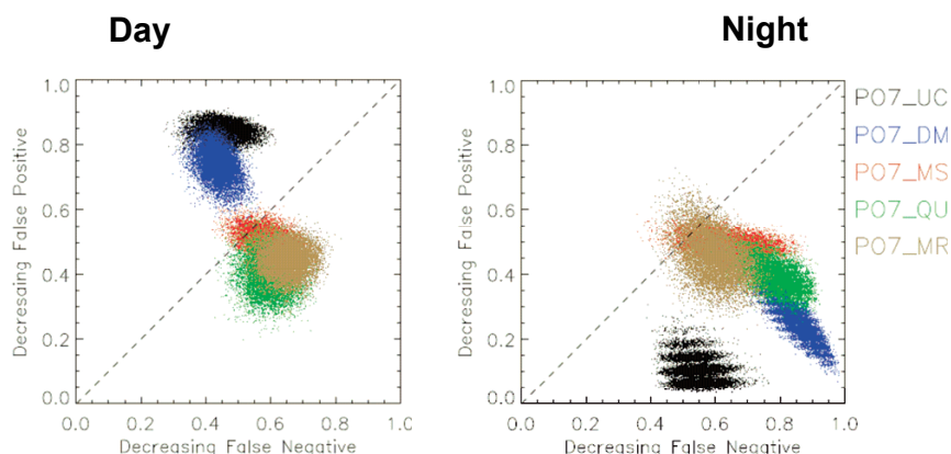
Figure 2. Comparisons of Bootstrap-Resampled User-Oriented Measure of Effectiveness (MOE) Values for Urban T&D Model Predictions of the 17 Daytime (Left) and 12 Nighttime (Right) Releases of JU03 Within the CBD Using the PO7 MET Input Option. The models represented are HPAC/Urban Canopy (UC), HPAC/UDM (DM), HPAC/MSS (MS), QUIC-URB/QUIC-PLUME (QU), and MESO/RUSTIC (MR). [MOE values nearer to the “perfect” value of (1,1) represent improved predictions; values “above” the diagonal line correspond to under-predictions, whereas values “below” the diagonal line correspond to over-predictions.]
