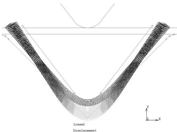
Figure 10. Displacement vector plot
