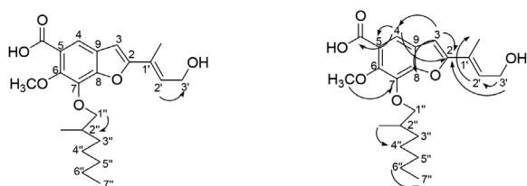
FIGURE 2. 2D NMR correlations of 2-[(1'E)-3'-hydroxyl-1'-methyl-1'-propen-1'-yl]-6-methoxy-7-[(2''-methylheptyl)oxy]-5-benzofuran-3-carboxylic acid, (a) COSY and (b) HMBC
