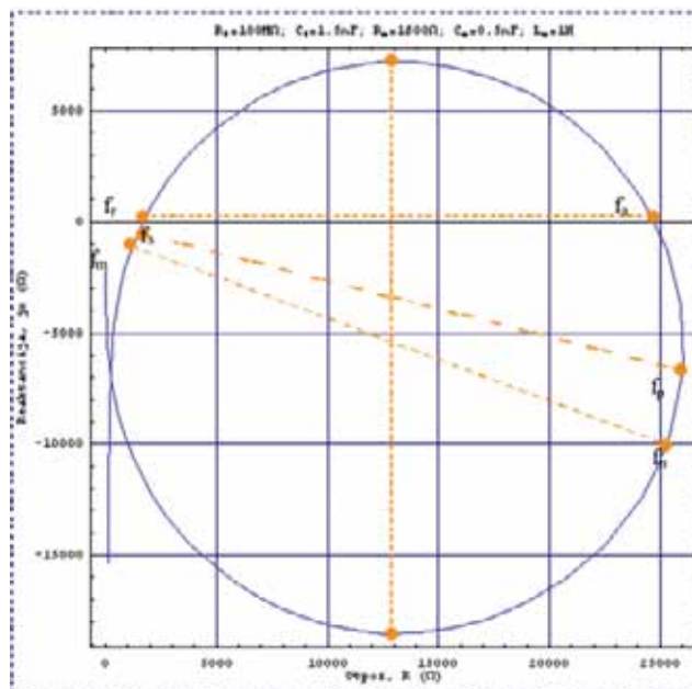
Figure 4 Illustration of electrical impedance of piezoelectric array elements in a complex plain with an outlined position of basic frequencies: f_r , f_a , f_m , f_n , f_s and f_p .
