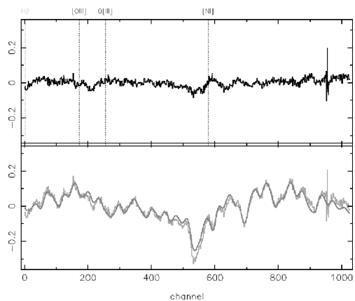
Figure 1. A typical example of the calculation of the derived kinematics for NGC 7768 with the MOVEL algorithm. In the lower panel, the smooth line corresponds to the optimal template spectrum, plotted together with the galaxy spectrum which has been shifted and broadened to the derived parameters. The upper panel shows the residuals of fit (in relative flux units), with the dotted lines indicating the positions of typical emission lines. This illustration spans 4900 to 5400 Å.
