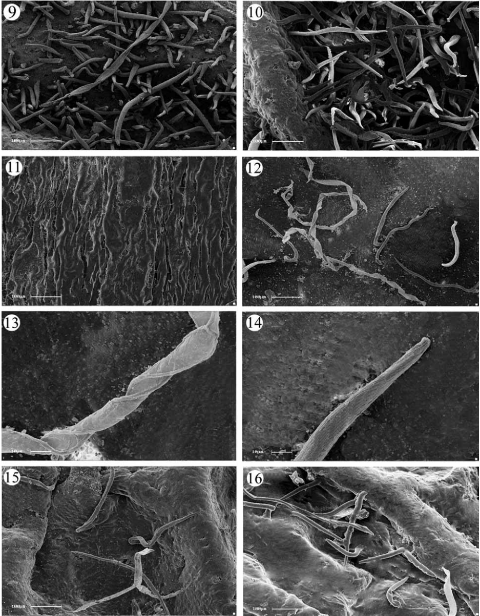
Plate 2. SEM micrographs of drupe pericarp indumentum of Iranian species of Amygdalus . 9 – A. carduchorum , 10 – A. elaeagnifolia subsp. elaegnifolia , 11 – A. reticulata , showing the glabrous pericarp, 12–14 – A. arabica , 15 – A. glauca , 16 – A. scoparia .
