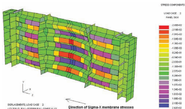
Figure 7 Prototype analysis – HC version - LC2 - \sigma_x membrane stresses (N/mm 2 ) Slika 7 Analiza prototipa – HC verzija - LC2 - \sigma_x membranska naprezanja (N/mm 2 )
