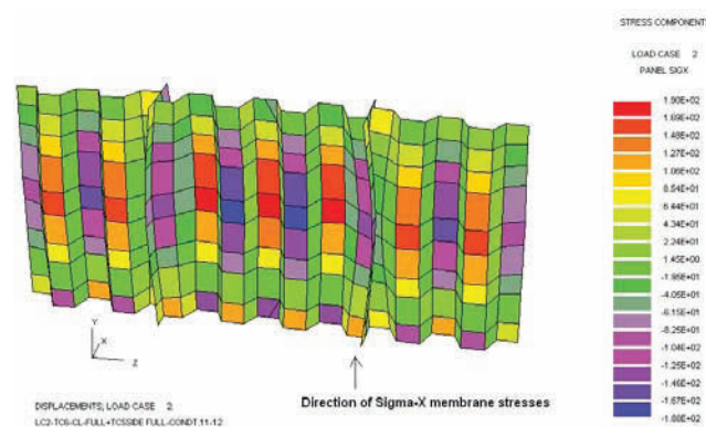
Figure 9 Prototype analysis – VC version - LC2 - \sigma_x membrane stresses (N/mm 2 ) Slika 9 Analiza prototipa – VC verzija - LC2 - \sigma_x membranska naprezanja (N/mm 2 )
