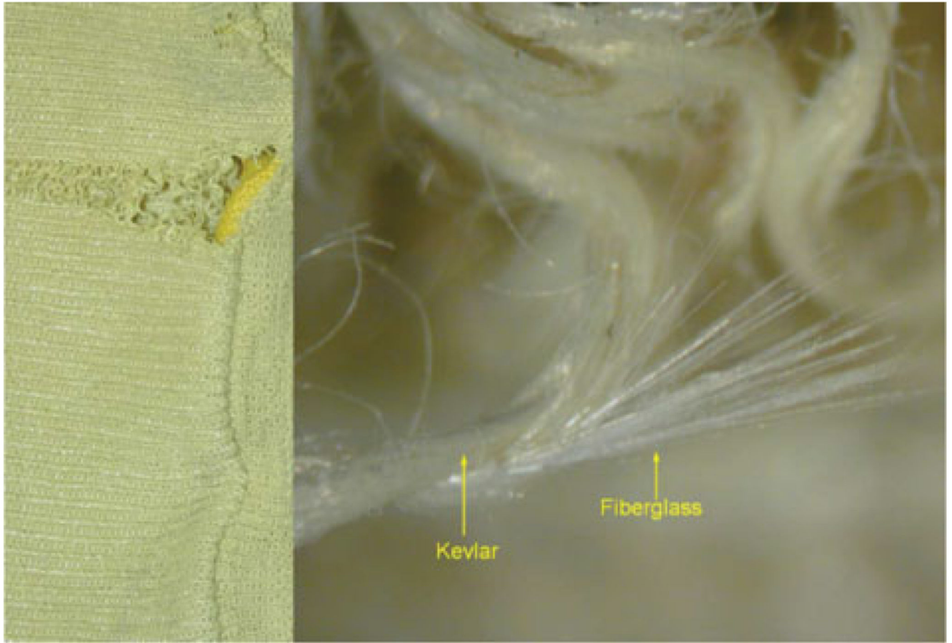
FIGURE 4. Photograph showing tear in laundered sleeve and broken fiberglass bundles in tear at 15×. (color figure available online)
