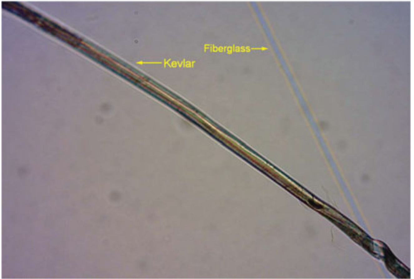
FIGURE 5. Photomicrograph showing Kevlar and fiberglass from sleeve at 200 \times . (color figure available online)
