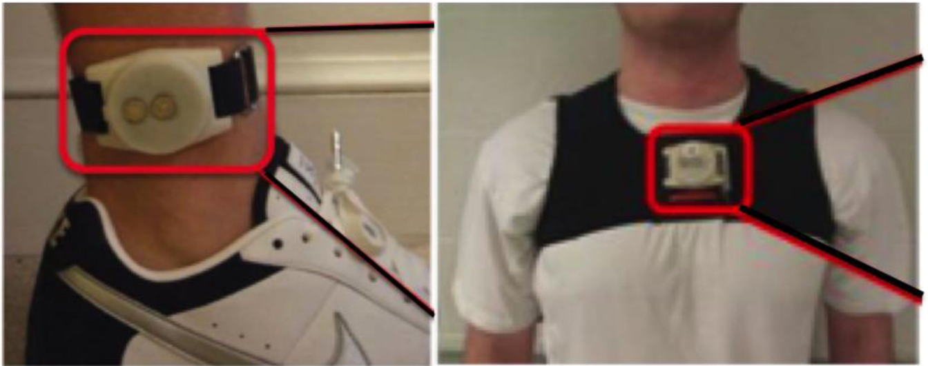
Figure 1. Attachment of IMU sensors at (a) shank and (b) sternum level using velcro strap.
