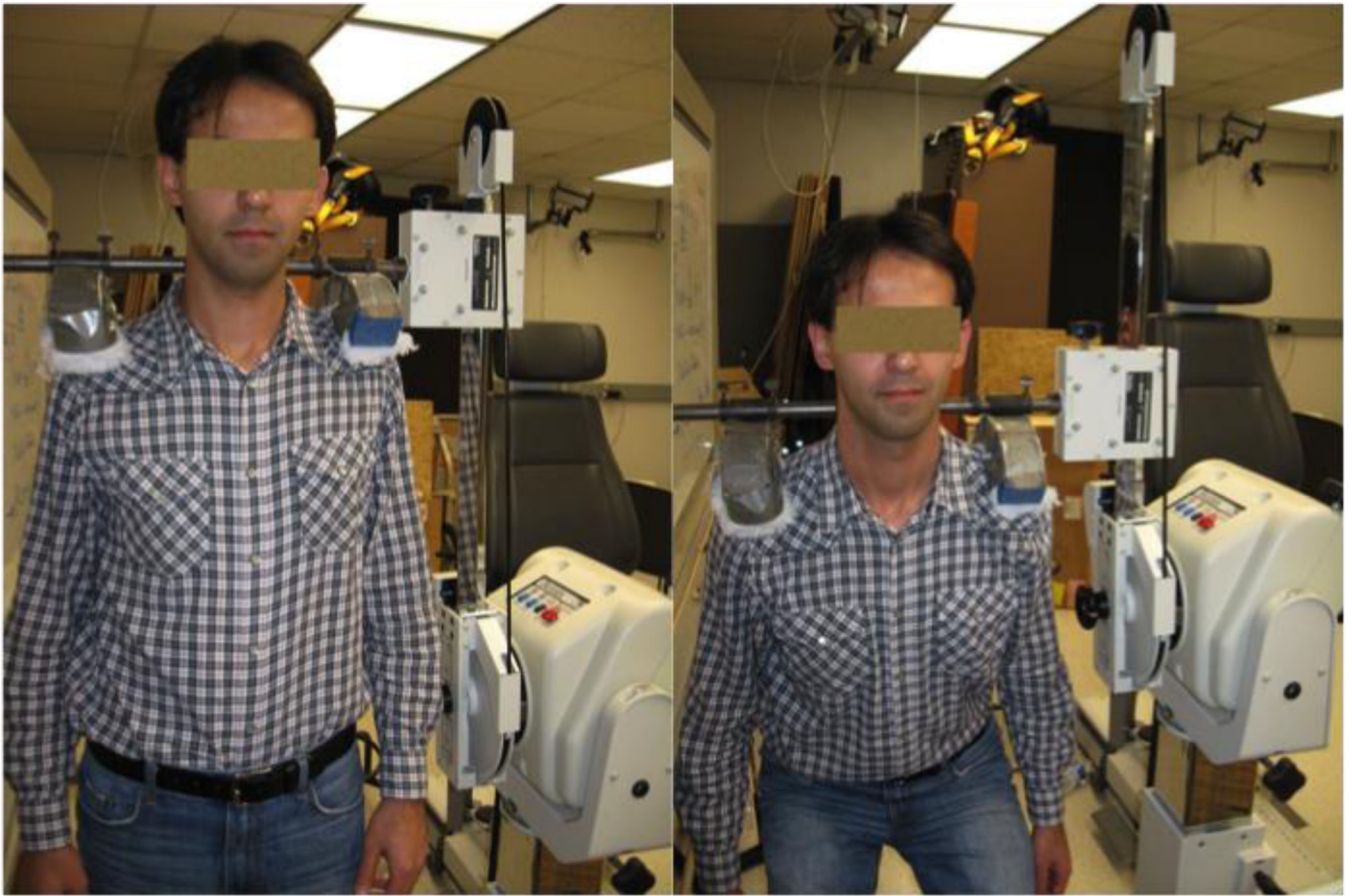
Figure 3. Customized Biodes attachment for measurement of maximum voluntary exertions.
