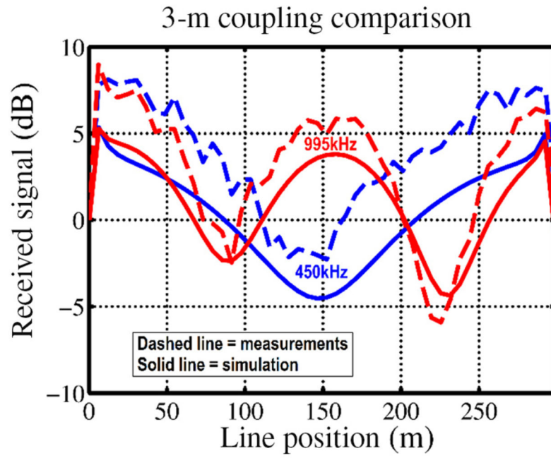
Fig. 12. Comparison of line-to-antenna-coupling measurement versus simulation.
