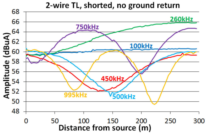
Fig. 8. LCD—two-wire TL, no ground connected.
