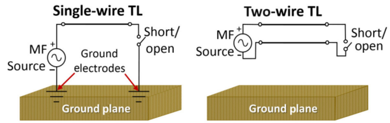
Fig. 6. TL test configurations.
