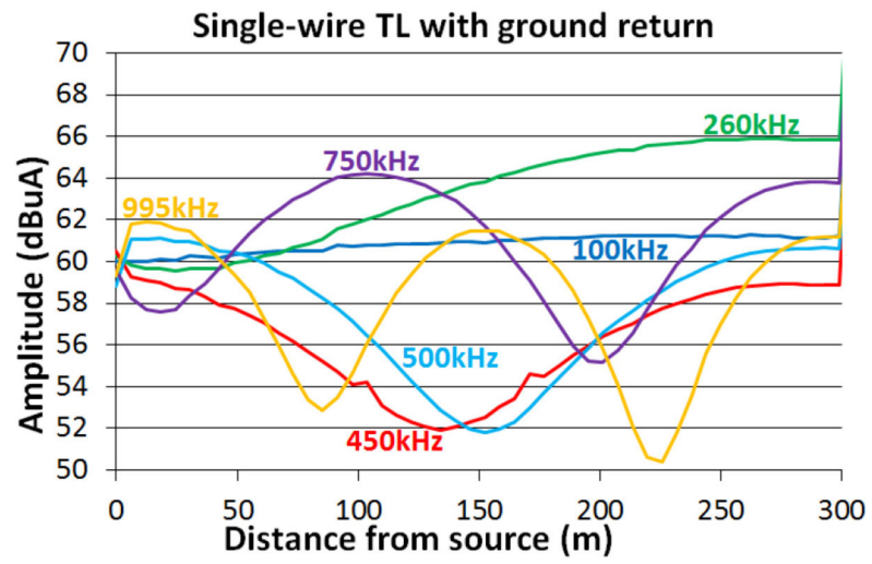
Fig. 9. LCD—single-wire TL, connected to ground.
