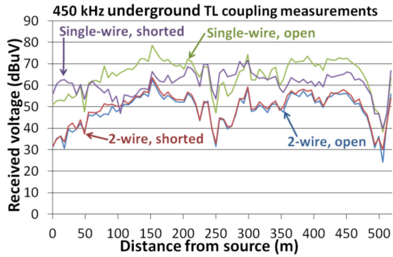
Fig. 14. Underground-coupling measurements at 450 kHz.
