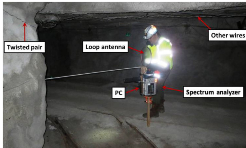
Fig. 13. Underground-transmission-line-coupling measurements.
