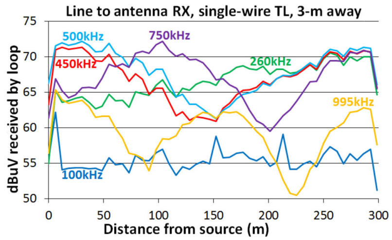
Fig. 11. Surface antenna coupling—single-wire TL, connected to ground.
