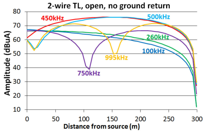
Fig. 7. LCD—two-wire TL, open, no ground connected.
