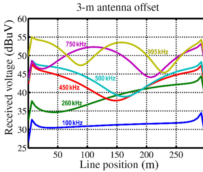
Fig. 4. Coupling simulation of a single conductor connected to ground.
