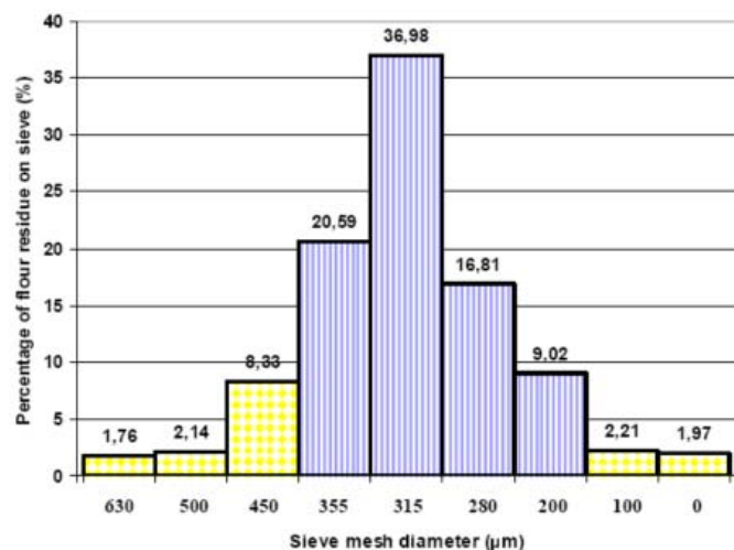
Figure 4. Results of sieving in time of 15 minutes (sample 12 CF-US)
