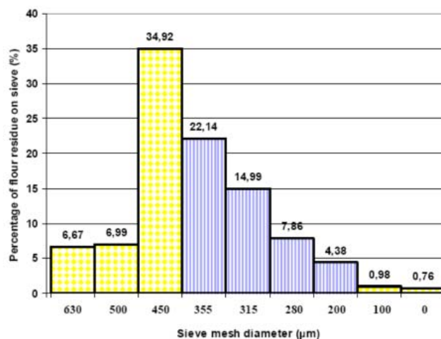
Figure 2. Results of sieving in time of 15 minutes (sample 3 CF)
