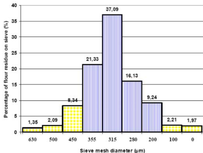
Figure 3. Results of sieving in time of 10 minutes (sample 9 CF-US)
