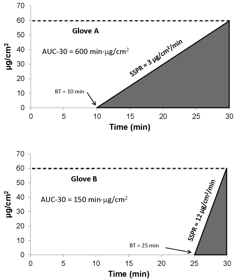
FIGURE 3. Comparison of cumulative permeation at 30 min (dotted line) vs. area under the curve at 30 min (AUC-30) for two scenarios where the permeation parameters are different, but the cumulative permeation amounts are the same. Based on the AUC-30, Glove B represents a 4-fold lower hazard potential for a 30-min exposure. BT = breakthrough time (min). SSPR = steady-state permeation rate (µg/cm 2 /min).
