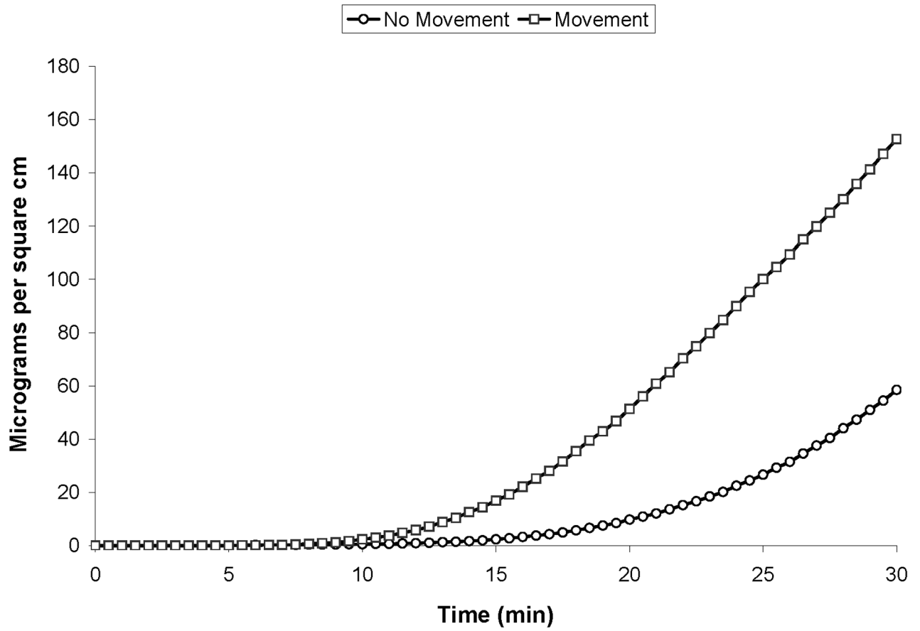
FIGURE 2. Exemplary permeation curves showing no movement and movement exposures for permeation of ethanol through a disposable nitrile glove product
