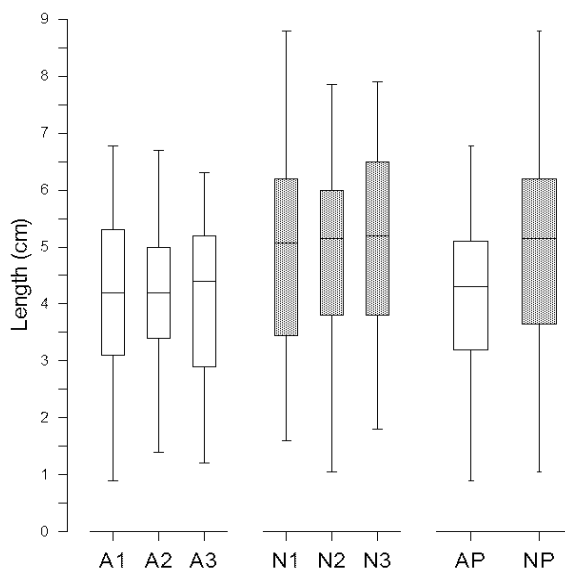
Fig. 1. Box-plots for the length of the date mussel Lithophaga lithophaga . A1, A2 and A3 are samples from artificial structures; N1, N2 and N3 are samples from natural structures. AP and NP are pooled samples for artificial and natural structures, respectively
