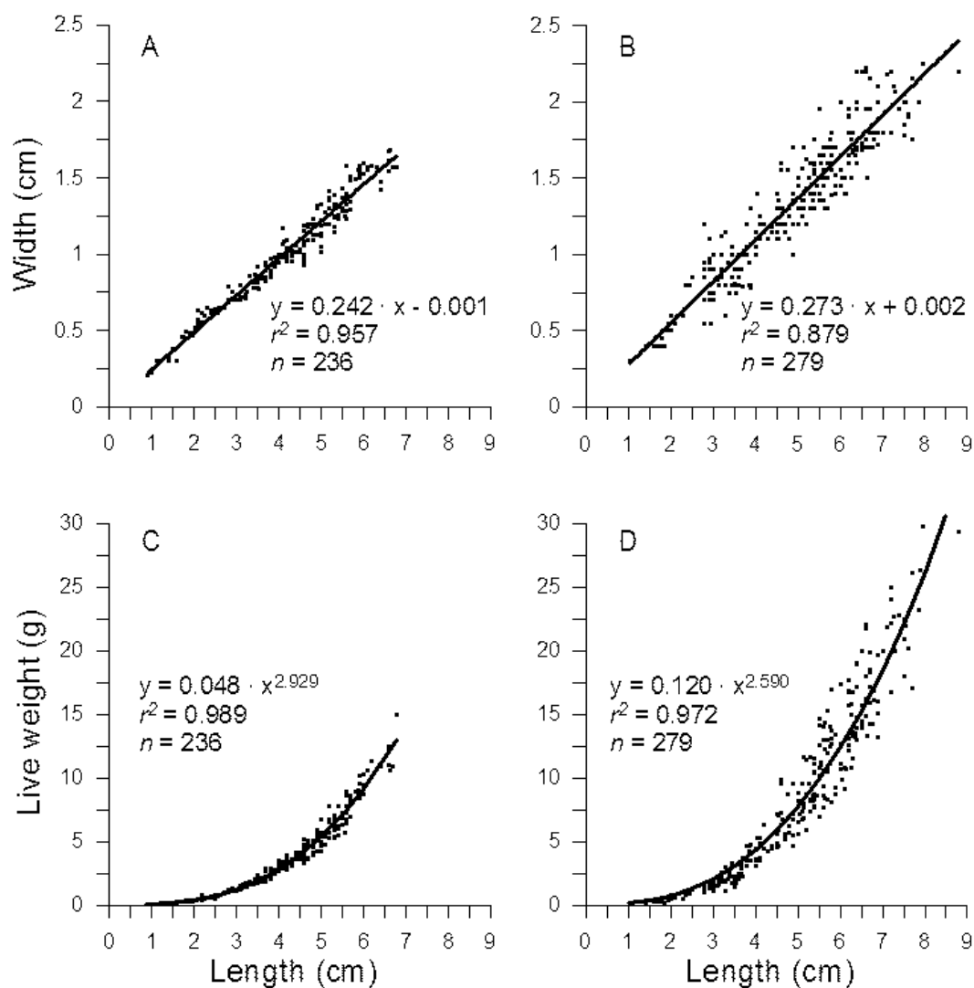
Fig. 2. Scatter-plots of width against length with linear regression line fitted for artificial (A) and natural structures (B), and of live weight against length with non-linear (allometric) regression line fitted for artificial (C) and natural structures (D) for date mussels Lithophaga lithophaga
