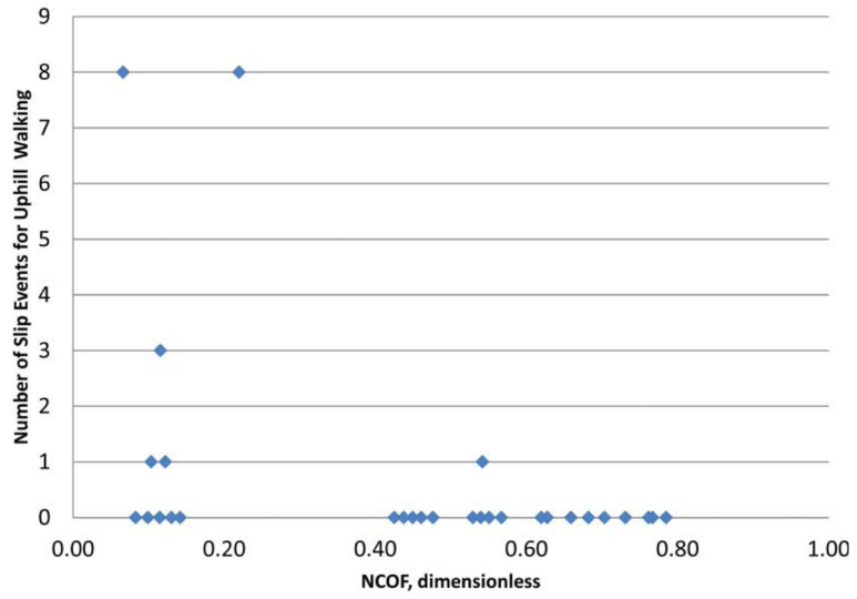
FIGURE 8. Number of slips for uphill walking trials by NCOF for all materials at all inclines with or without contaminants. NCOF values shown are for all walkway materials and angles.
