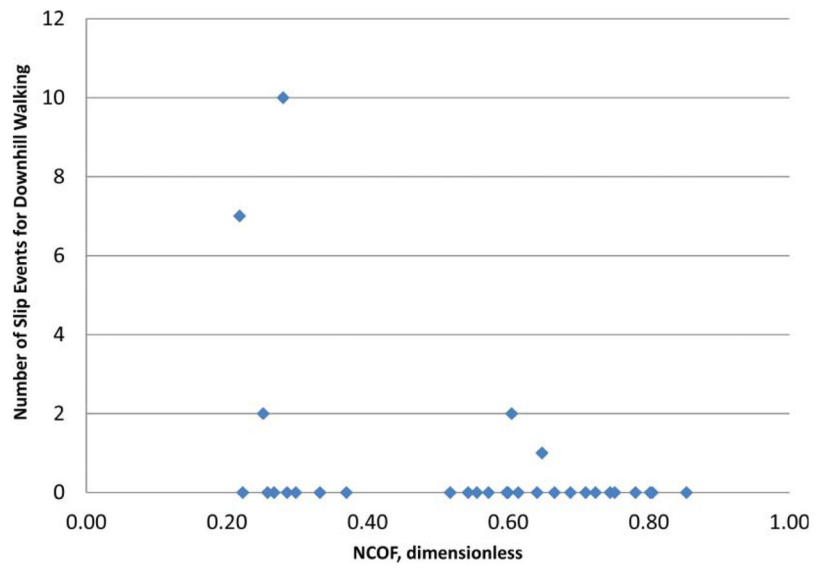
FIGURE 9. Number of slips for downhill walking trials by NCOF for all materials at all inclines with or without contaminants. NCOF values shown are for all walkway materials and angles.
