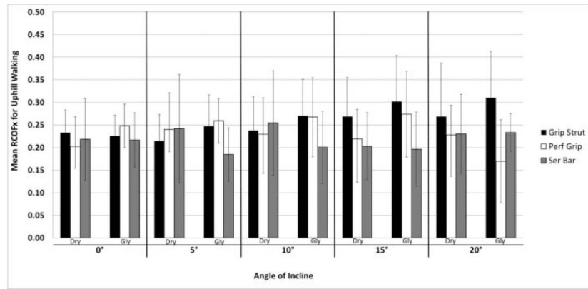
FIGURE 6. Mean RCOF x measures for uphill walking on dry and glycerol contaminated (Gly) walkways at the five angles of incline. Error bars denote one standard deviation. Results are presented for those trials in which the participants did not slip.
