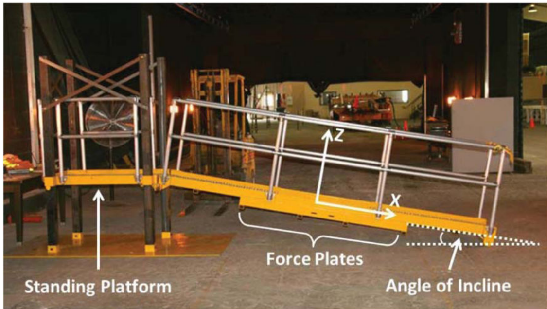
FIGURE 5. Instrumented walkway used in the study showing the standing platform and location of force plates.
