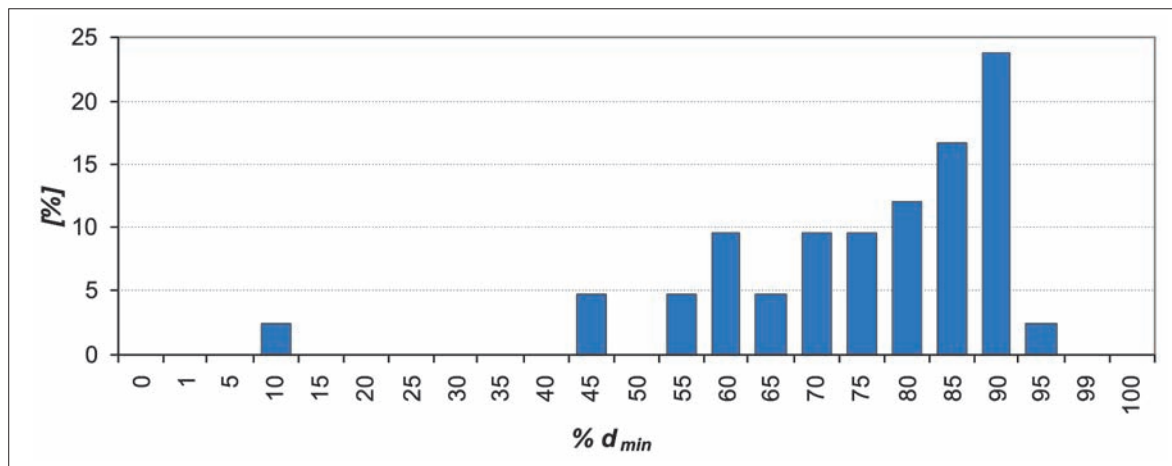
Diagram 2 Percentage of some percentiles of minimal diameter in the assessment of location parameter ( a ) of the Weibull model of diameter structure.
