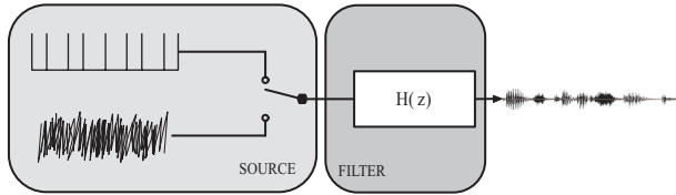
Fig. 2. The source-filter model.
