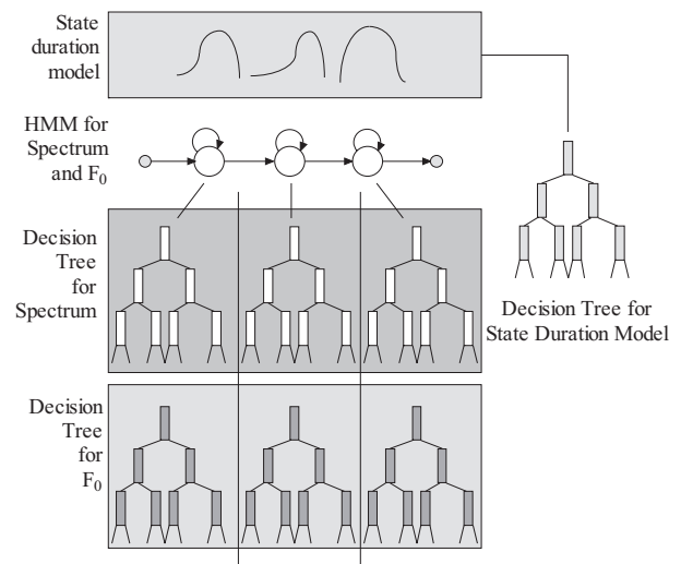
Fig. 5. Decision trees for spectrum, pitch and duration.
