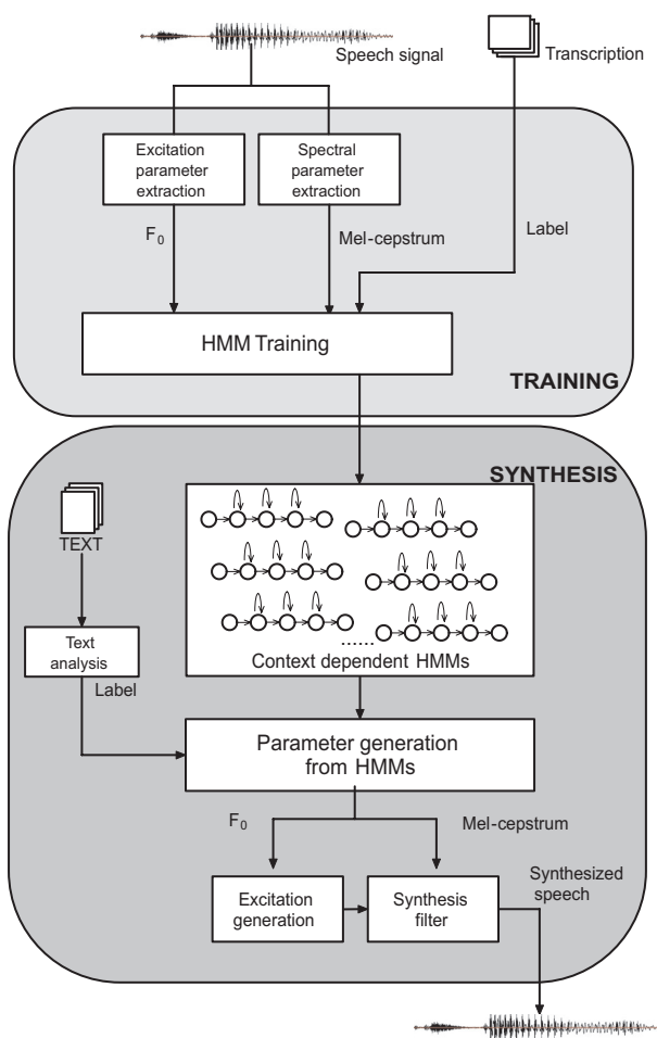
Fig. 1. Overview of the HMM speech synthesis.
