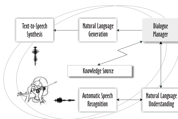
Figure 1. Natural-language dialogue system.
