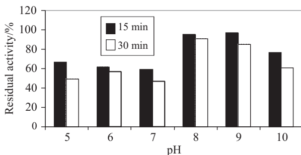
Fig. 6. Stability of endoglucanase at various pH. Enzyme preparation was incubated at 45 °C with different buffers for 15 and 30 min and residual activity was determined (original activity was 2290 U/L). Data represent the mean of three replicates
