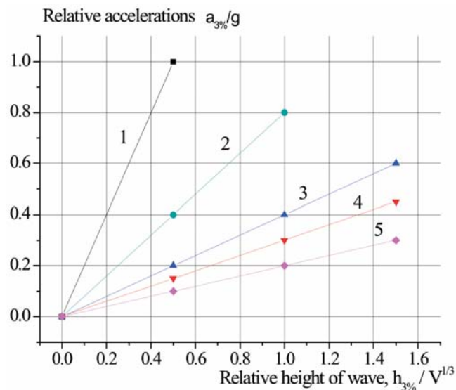
Figure 3 Relative vertical acceleration at the mass centre: 1 – monohull plane boats; 2 – air cushion boats; 3 – “wave-piercing” catamarans; 4 – SWA boats; 5 – boats with deeply submerged and automatically controlled foils
