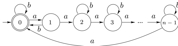
Fig. 1 An n -state dfa of a language L that does not have the empty quotient.
