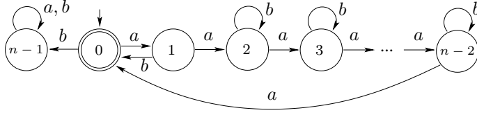
Fig. 2 An n -state dfa of a language L that has the empty quotient.
