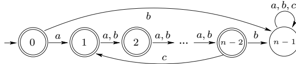
Fig. 5 An n -state dfa of prefix-closed language L .
