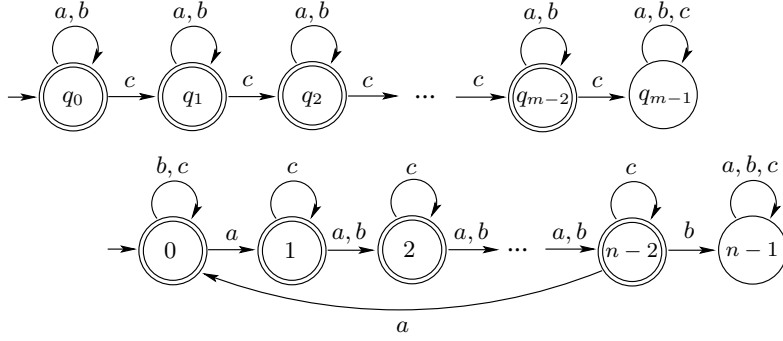
Fig. 3 Dfa's of prefix-closed languages K (top) and L (bottom).
