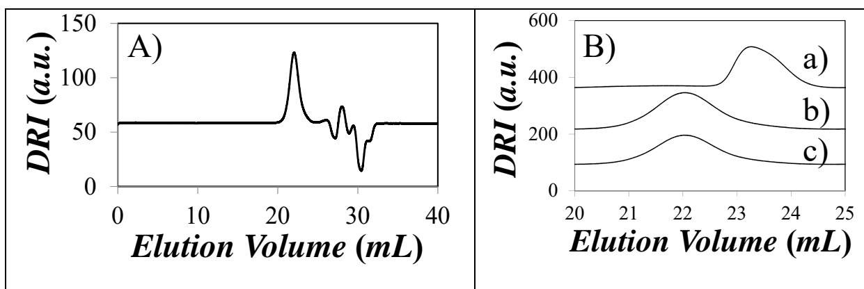
Figure 5. A) GPC trace for purified PEG 113 - b -PMEO 2 MA 77 . B) Zoomed-in GPC traces for (a) the macroinitiator, (b) the unpurified PEG 113 - b -PMEO 2 MA 77 sample, and (c) the purified PEG 113 - b -PMEO 2 MA 77 sample.
