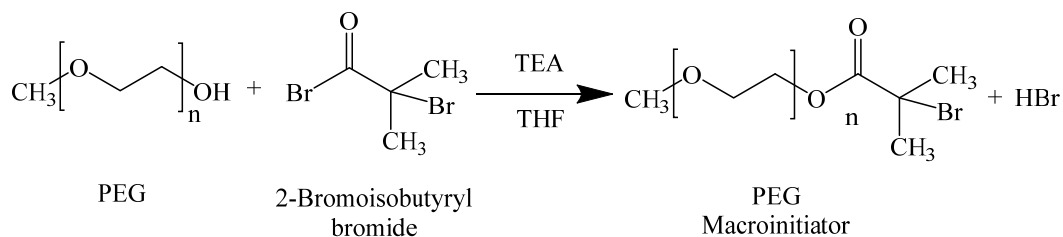
Scheme 1: Synthesis of PEG macroinitiator. 16,18
