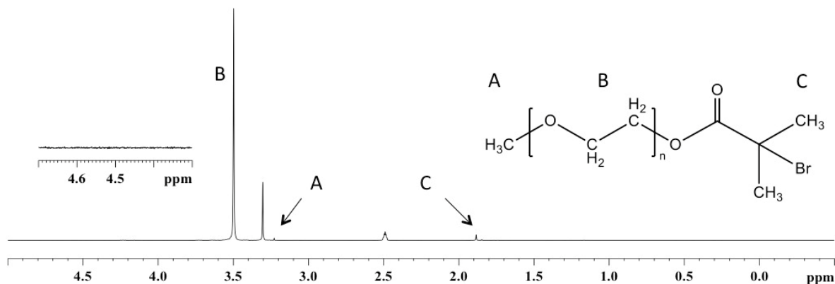
Figure 3. ^1\text{H} NMR spectrum of the purified 2-bromoisobutyrate PEG macroinitiator together with peak assignment. The small peak at 2.5 ppm is for DMSO. [Poly] = 20 mg/mL.
