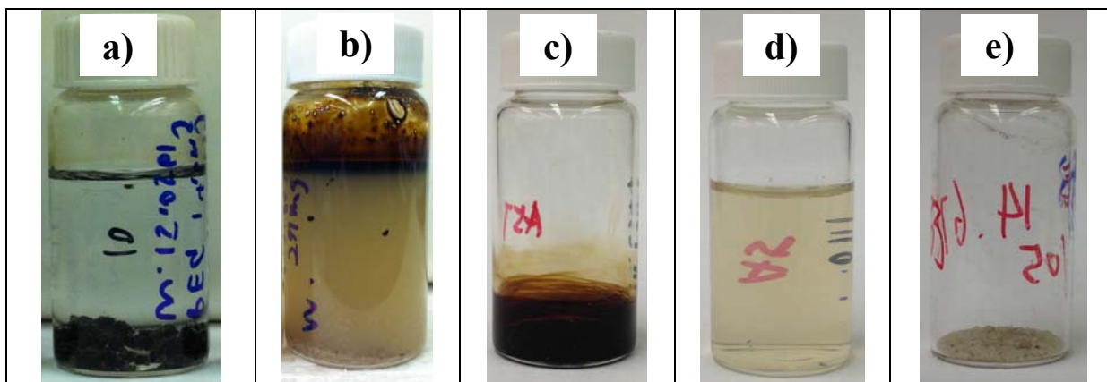
Figure 2. a) Before extraction: Mixture of oil sand particles at the bottom, 15 mL of 1 mg/mL PEG 113 - b -PMEO 2 MA 77 aqueous solution, and 60 mg of toluene on top of the solution. After 24 hrs extraction at T = 45 °C: b) Mixture with the extracted oil at the top of the aqueous solution; c) Oil recovered from the extraction; d) PEG 113 - b -PMEO 2 MA 77 aqueous solution; e) Pristine sand particles.
