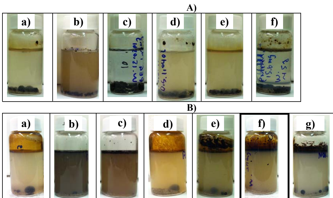
Figure 8. A) Extraction without toluene: a) pure water, b) 100 mM SDS, and 1 mg/mL aqueous solutions of c) PEG, d) PMEO 2 MA, e) PEG 113 - b -PMEO 2 MA 77 , and f) PNIPAM. B) Extraction with 60 mg toluene: a) pure water, b) 100 mM SDS, c) 200 mM SDS, and 1
