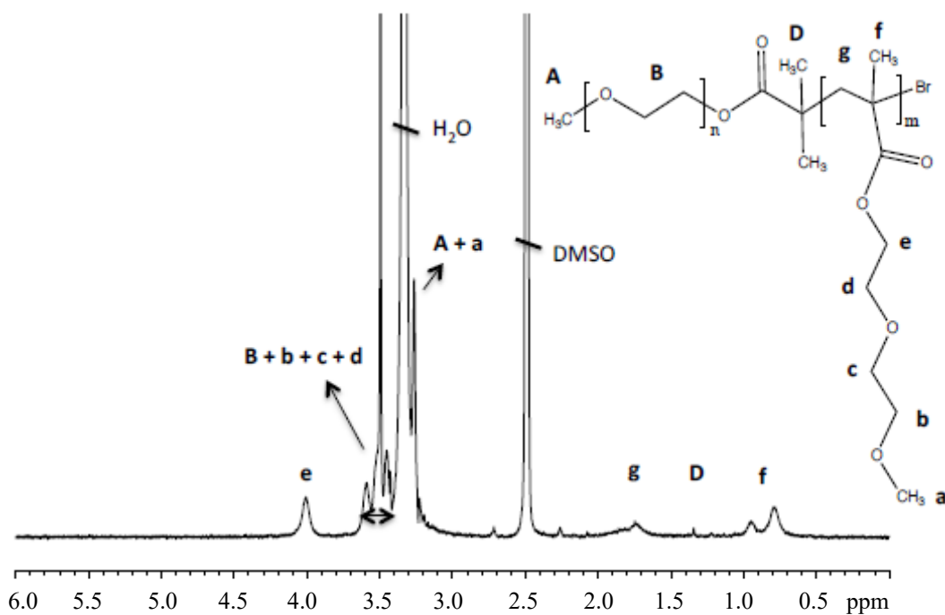
Figure 4. Chemical structure and ^1\text{H} NMR spectrum of PEG 113 - b -PMEO 2 MA 77 .
