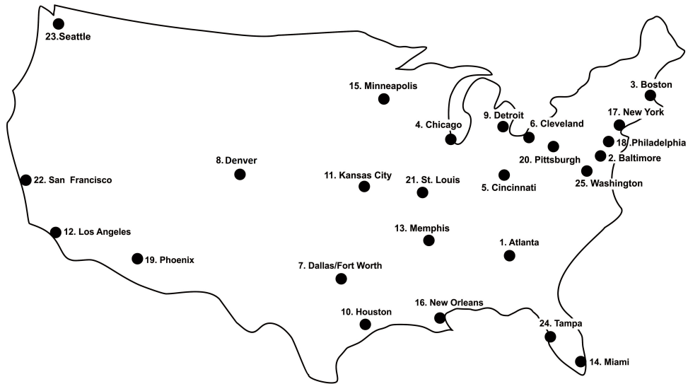
Figure 4.1: CAB dataset.
