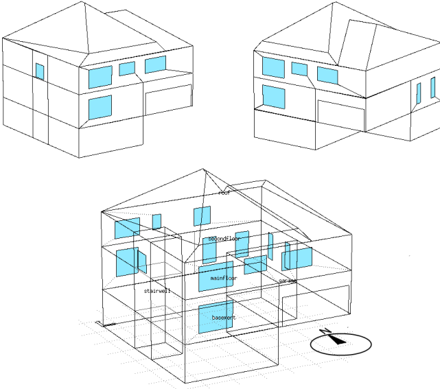
Figure 1: Geometry of CCHT house model in ESP-r (windows shaded blue).
