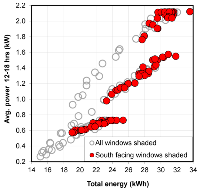
Figure 8: Total cooling energy vs. averaged power between 12:00-18:00 hours showing all results for the completely shaded façade (unfilled markers) and the partially shaded cases with shading on the south facing windows only (filled markers).
