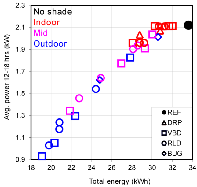
Figure 5: Total cooling energy vs. averaged power between 12:00-18:00 hours for the set of shading configurations and zoned control scenario C0 (shade layer position indicated by colour).
