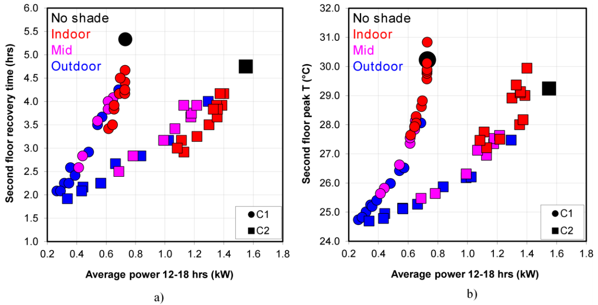
Figure 7: Averaged power between 12:00-18:00 hours vs. a) second floor recovery time and b) second floor peak temperature for zoned control scenarios C1 and C2 (shade layer position indicated by marker colour).
