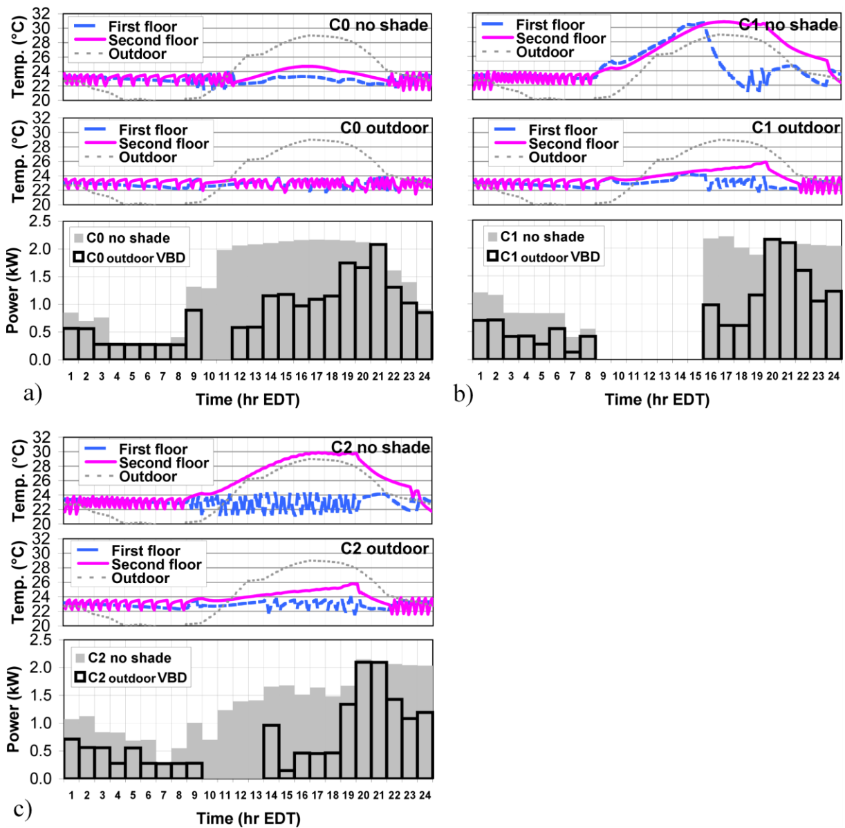
Figure 4: Temperatures and hourly averaged cooling power for unshaded vs. outdoor Venetian blind cases subject to the three zoned control scenarios a) C0, b) C1 and c) C2.
