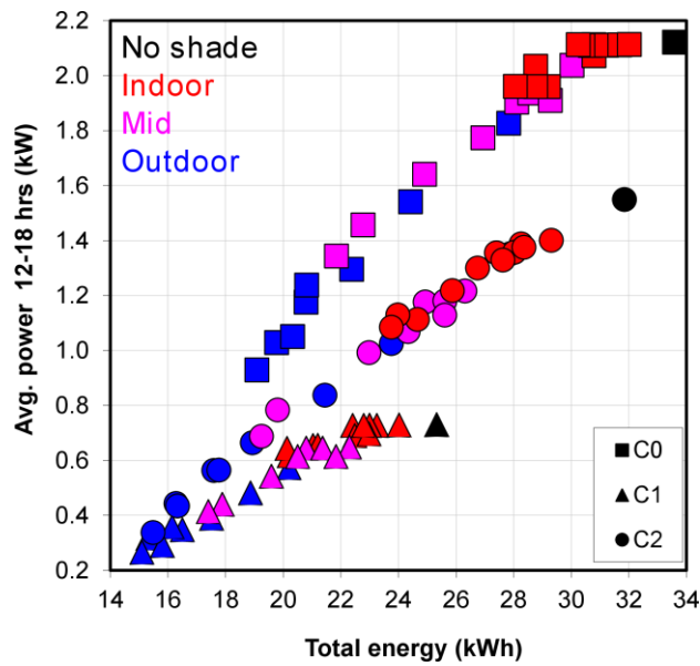
Figure 6: Total cooling energy vs. averaged power between 12:00-18:00 hours for the set of shading configurations and zoned control scenarios C0, C1 and C2 (shade layer position indicated by marker colour).
