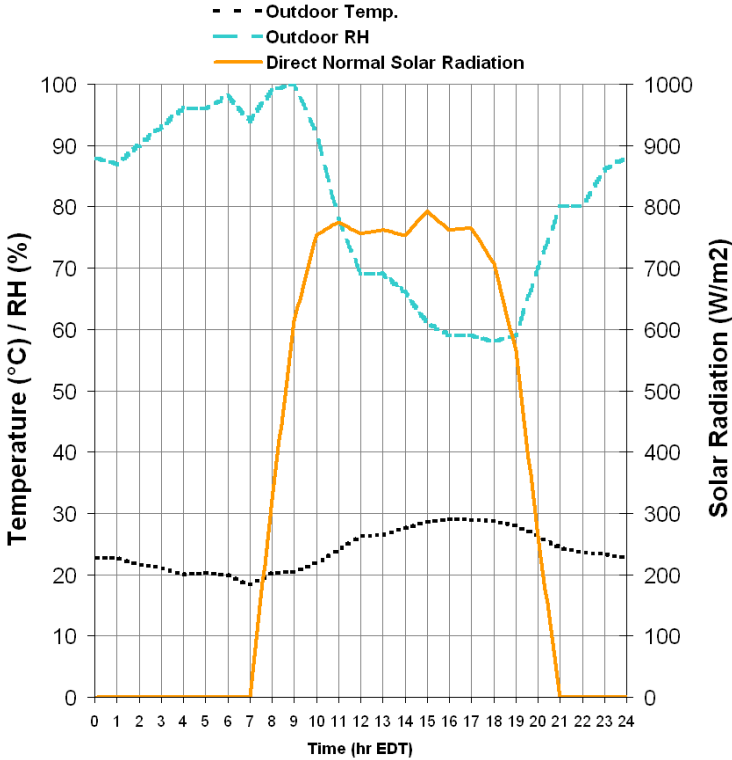
Figure 2: Weather data used in the ESP-r model. Data is from August 31 st , 2000, Toronto.
