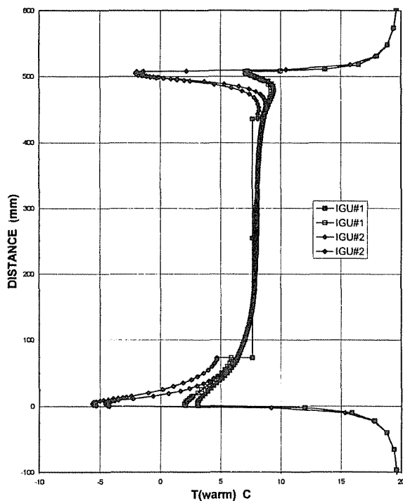
Figure 3 Effect of spacer material, foam vs. metal, IGUs 1 and 2 (BRAVO-closed symbols, VISION4/FRAVE 4.0-open symbols).
