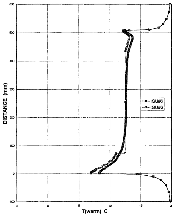
Figure 9 Triple glazing with 12.7-mm (.5-in.) pane spacing, IGU 6 (BRAVO-closed symbols, VISION4/FRAME 4.0-open symbols).
