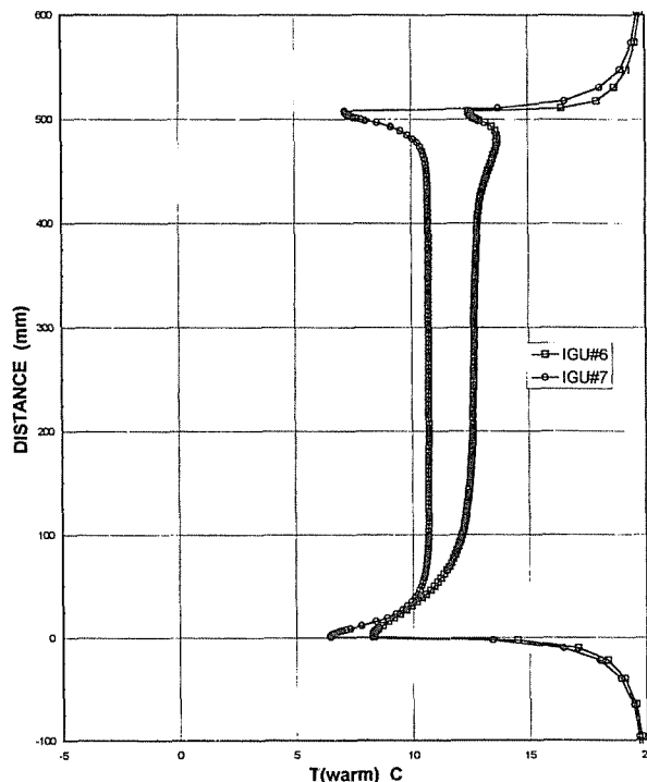
Figure 8 Comparison of triple-glazed units, IGUs 6 and 7 (BRAVO only).
