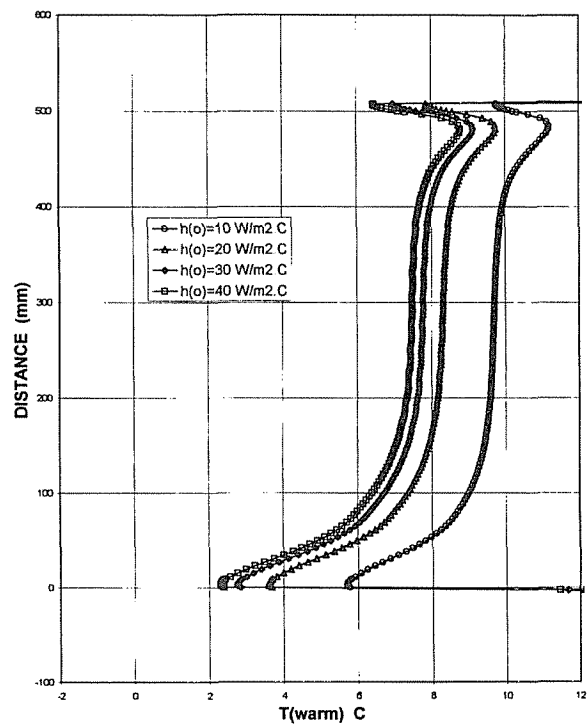
Figure 11 Sensitivity analysis: Effect of changes in h_o with h_i fixed at 8 \text{ W/m}^2 \cdot ^\circ\text{C} IGU 1 (BRAVO only).
