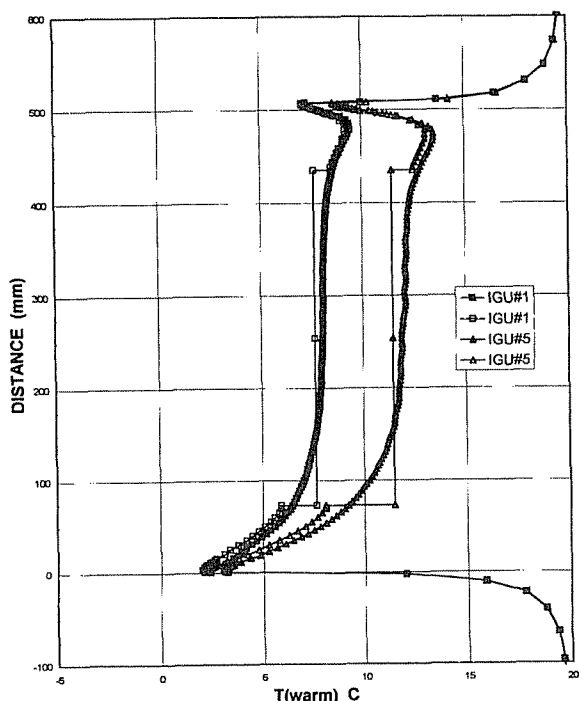
Figure 7 Effect of low-e coating, IGUs 1 and 5 (BRAVO-closed symbols, VISION4/FRAME 4.0-open symbols).
