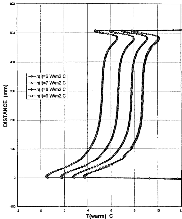
Figure 10 Sensitivity analysis: Effect of changes in h_i with h_o fixed at 30 \text{ W/m}^2 \cdot ^\circ\text{C} IGU 1 (BRAVO only).
