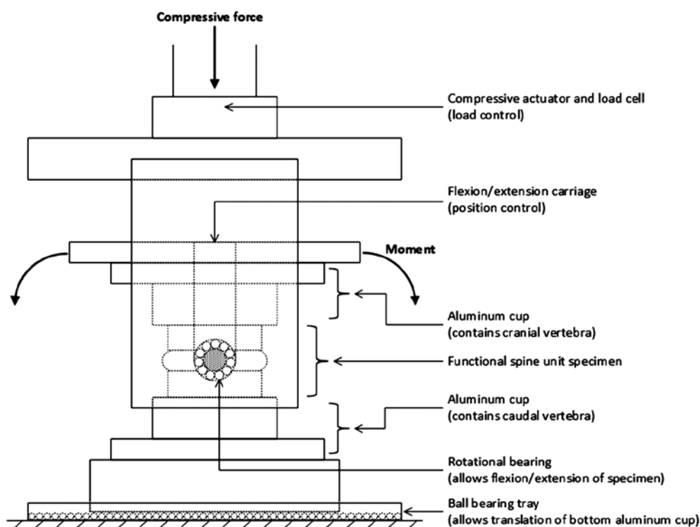
Figure 1. A schematic of the material testing system set-up.
