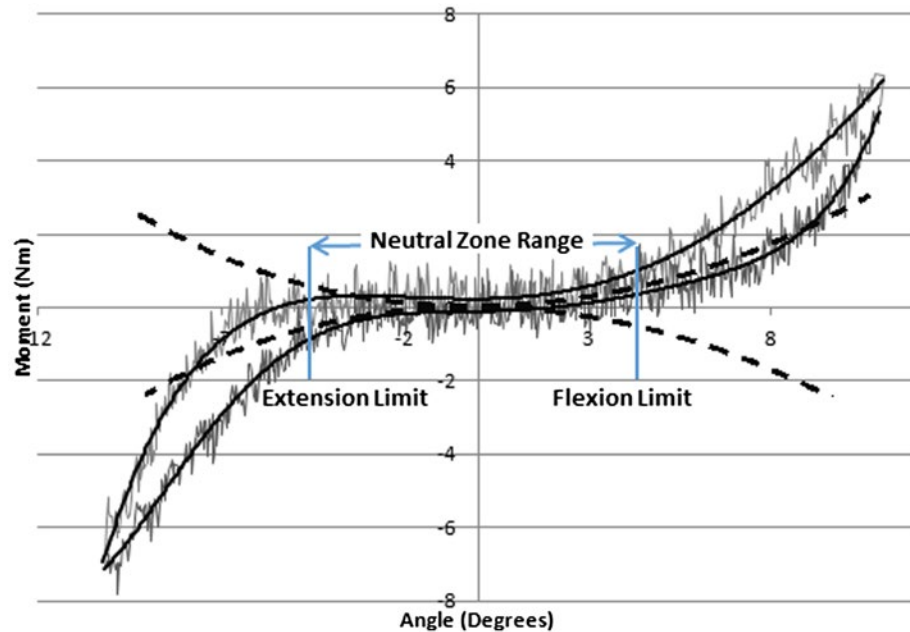
Figure 3. Defining neutral zone range using a method of fitting a fourth-order polynomial curve to the ascending and descending curve (solid line) to the raw data (thin line), and first derivative of the fitted curve (dotted line) was calculated (Thompson et al., 2003). The neutral zone range was defined by the angle where it reached \pm 0.05 Nm/degree (flexion and extension limit defined).
