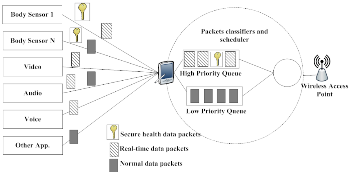
Figure 3.6: Traffic scheduling at PDA
