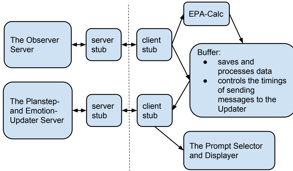
Figure 3.8: System design with server-client models
