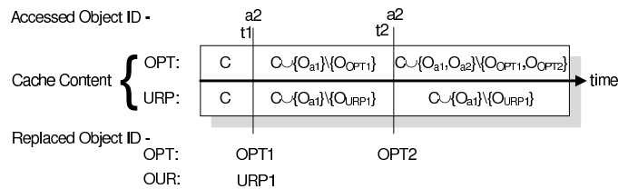
Figure C.1: Replacement in OUR and other policies
