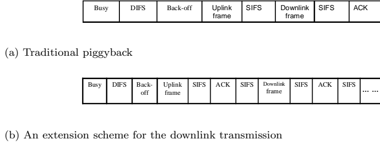
Figure 4.9: Bidirectional Transmission
