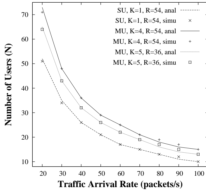
Figure 4.20: Maximum Number of Users under Various Traffic Arrivals
