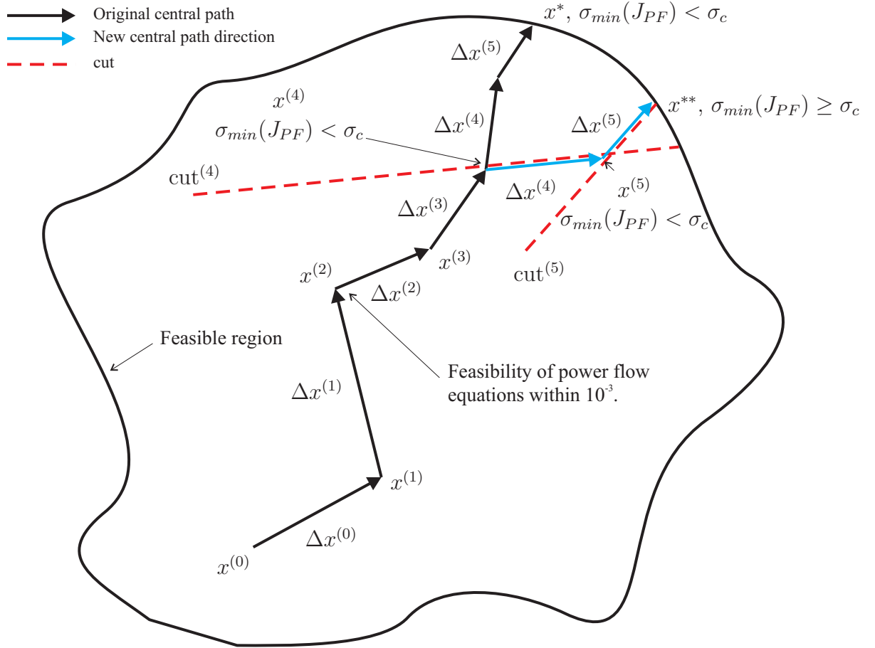
Figure 5.1: Graphic representation of the proposed CP/IPM algorithm.
