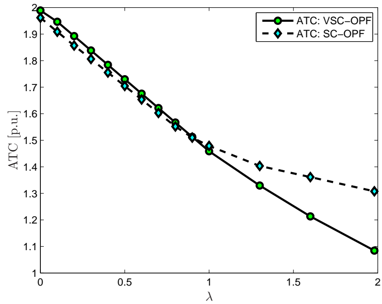
Figure 4.28: ATC with respect to system loading for the 6-bus system.
