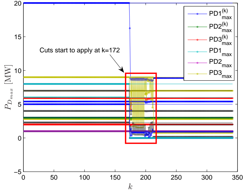
Figure 5.17: The box encloses the iterations at which some cuts are added in the CP/IPM when solving CIGRE-32 system.
