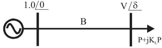
Figure 3.4: Generator-Infinite Bus system
