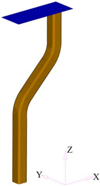
Figure 23: Finite element mesh of the crash model
