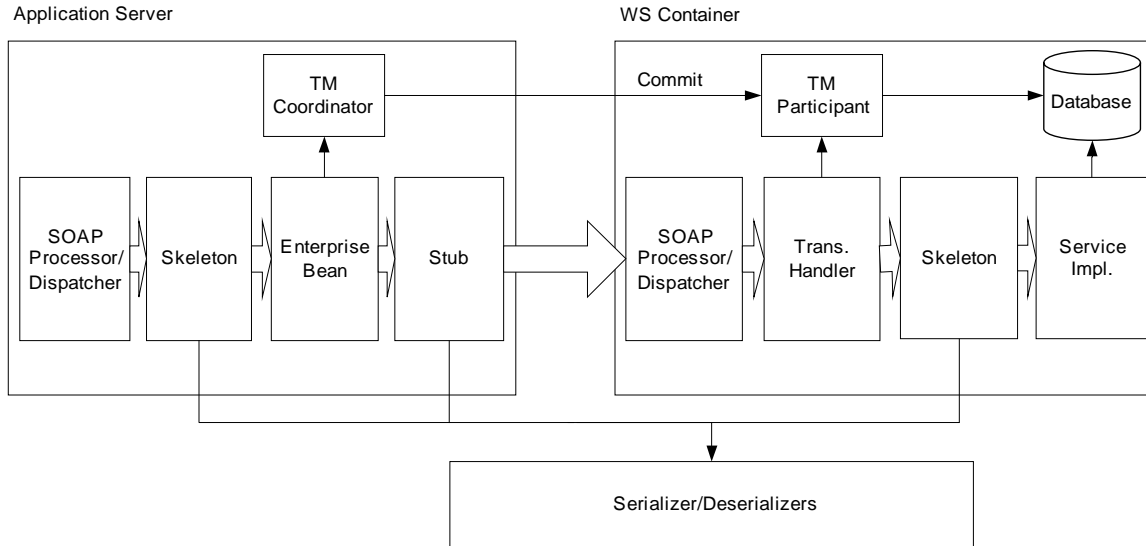
Figure 4. 9 Transaction Management in the Reference Architecture
