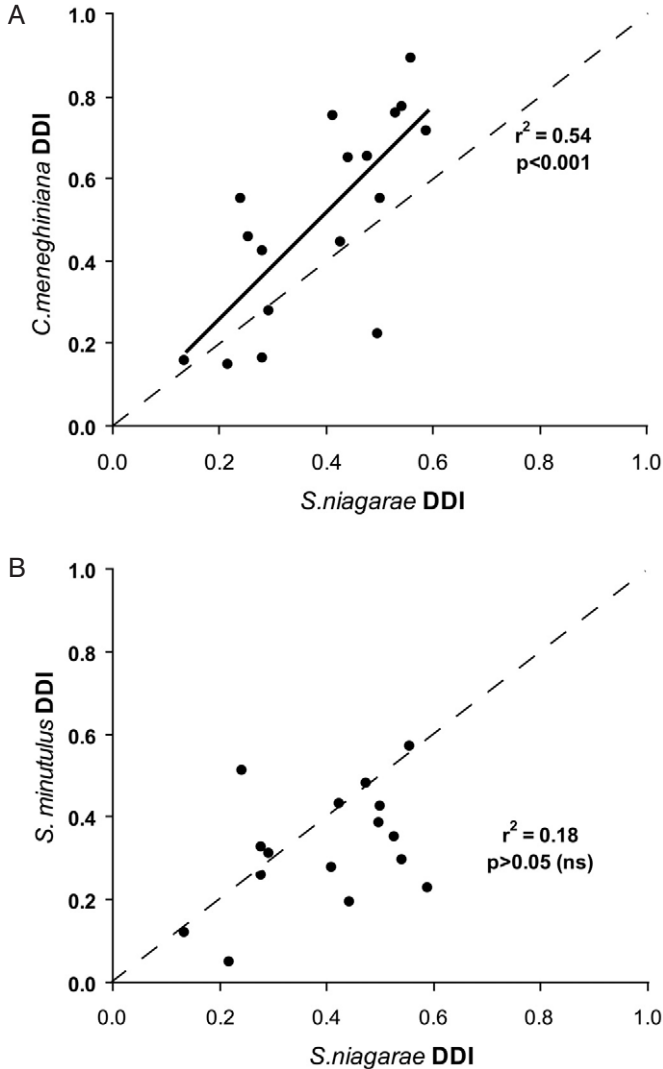
Fig. 3. Correlations between DDI (diatom dissolution index) scores for the 3 dominant taxa from Spiritwood Lake short core SW1. Increasing values indicate poorer preservation for DDI (in contrast to the F index). The dotted line shows the 1:1 line of equal preservation. (A) Stephanodiscus niagarae against Cyclotella meneghiniana ; (B) Stephanodiscus niagarae against Stephanodiscus minutulus complex.
