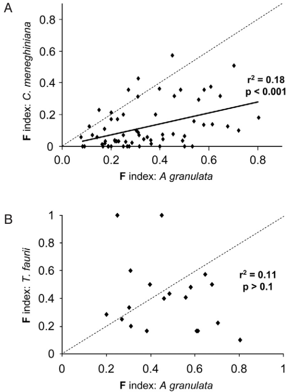
Fig. 6. Correlations between the F index scores for dominant taxa from the Lake Qarun core QARU2. Decreasing values indicate poorer preservation for the F index (in contrast to DDI). The dotted line shows the 1:1 line of equal preservation. (A) Aulacoseira granulata against Cyclotella meneghiniana ; (B) Aulacoseira granulata against Thalassiosira faurii . The significant correlation between F index scores in (A) and the trend (solid) line is indicated.
