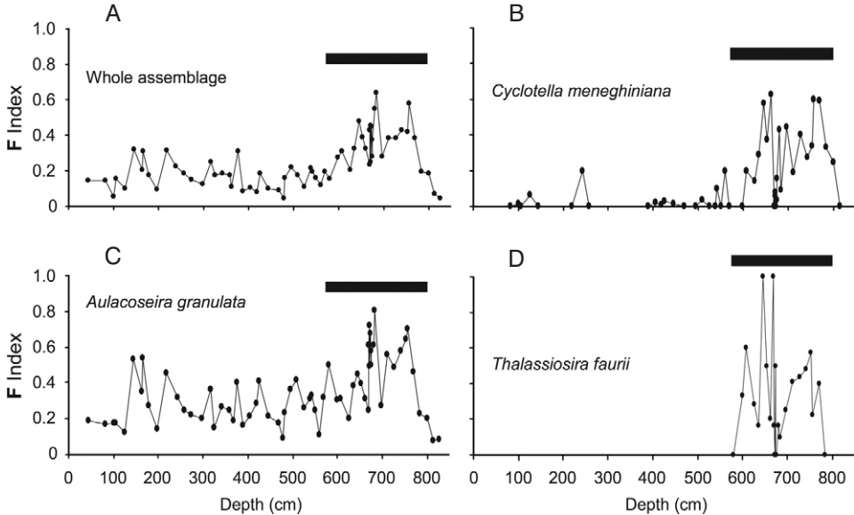
Fig. 5. Graphs A–D show the down-core (QARU2) variations in F index values for the (A) total diatom assemblage, (B) Cyclotella meneghiniana , (C) Aulacoseira granulata , and (D) for Thalassiosira faurii , respectively (see text). Solid bars indicate core sections with good valve preservation.
