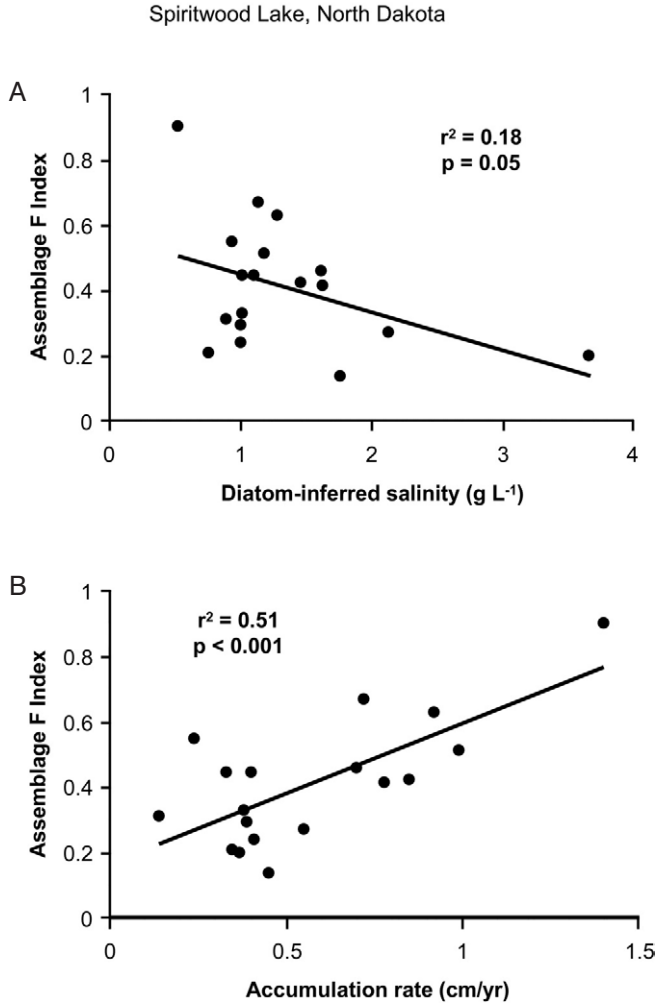
Fig. 2. Spiritwood Lake short core SW1. Scatter plots of (A) assemblage F index and diatom-inferred salinity (using the original NGP model of FRITZ, 1990, FRITZ et al., 1993, not adjusted for dissolution data) and (B) assemblage F index and accumulation rate (cm yr -1 ).
