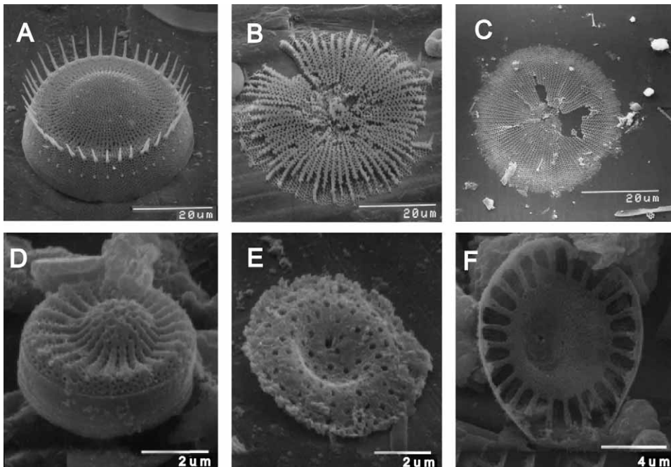
Fig. 1. SEM micrographs of diatoms common in the Spiritwood Lake short core, across a range of preservation states («dissolution stages»). (A)–(C): Stephanodiscus niagarae (A: pristine = stage 1, B: dissolved valve, stage 2, C: dissolved valve, stage 3). (D)–(E): Stephanodiscus minutulus (D: pristine, E: dissolved valve, stage 3). (F): Cyclotella meneghiniana , dissolved valve: stage 2. Adapted from Supplementary Material in RYVES et al. (2009).
