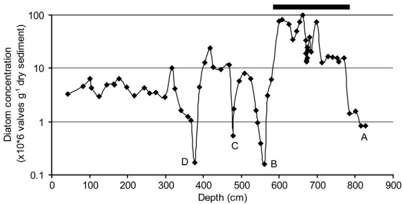
Fig. 8. Diatom concentrations in QARU2 plotted on a log scale to show four (A–D) very low diatom abundance zones (Tab. 2) which fall below the range where valve concentration and poor preservation are related (see Fig. 7). The solid bar indicates the core section with good valve preservation.
