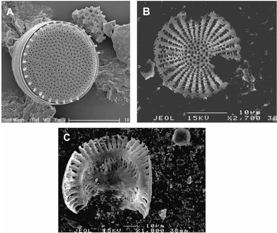
Fig. 4. SEM micrographs of diatoms extracted from a sediment core from Lake Qarun (QARU2, see text). (A): a near pristine valve of Thalassiosira faurii sampled from around 670 cm depth in the core; (B): a valve of Cyclostephanos dubius (though identification is hampered by dissolution) from around 420 cm in the core with extensive dissolution features; (C): a Campylodiscus valve from around 420 cm depth in the core showing marginal dissolution features (note, the Cyclotella meneghiniana valve central area in the top right of this image; dissolution stage 4).
