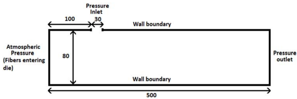
Figure 2: Geometry and boundary conditions of the computational domain. Note that lengths are given in mm.
