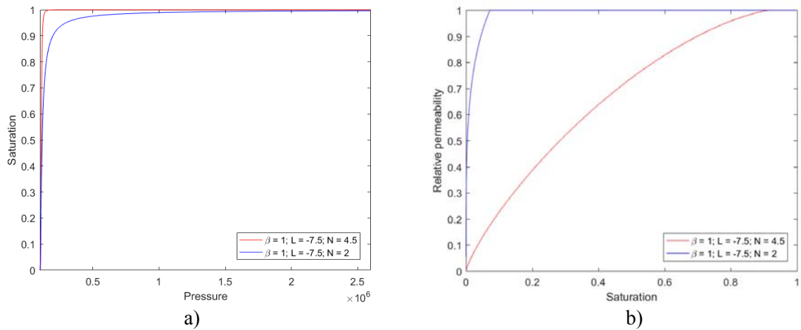
Figure 3: a) Saturation curves and b) relative permeability curves.
