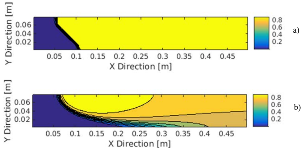
Figure 5: Stationary saturation fields for the two scenarios: a) \beta = 1 ; L = -7.5 ; N = 4.5 ; and b) \beta = 1 ; L = -7.5 ; N = 2 .
