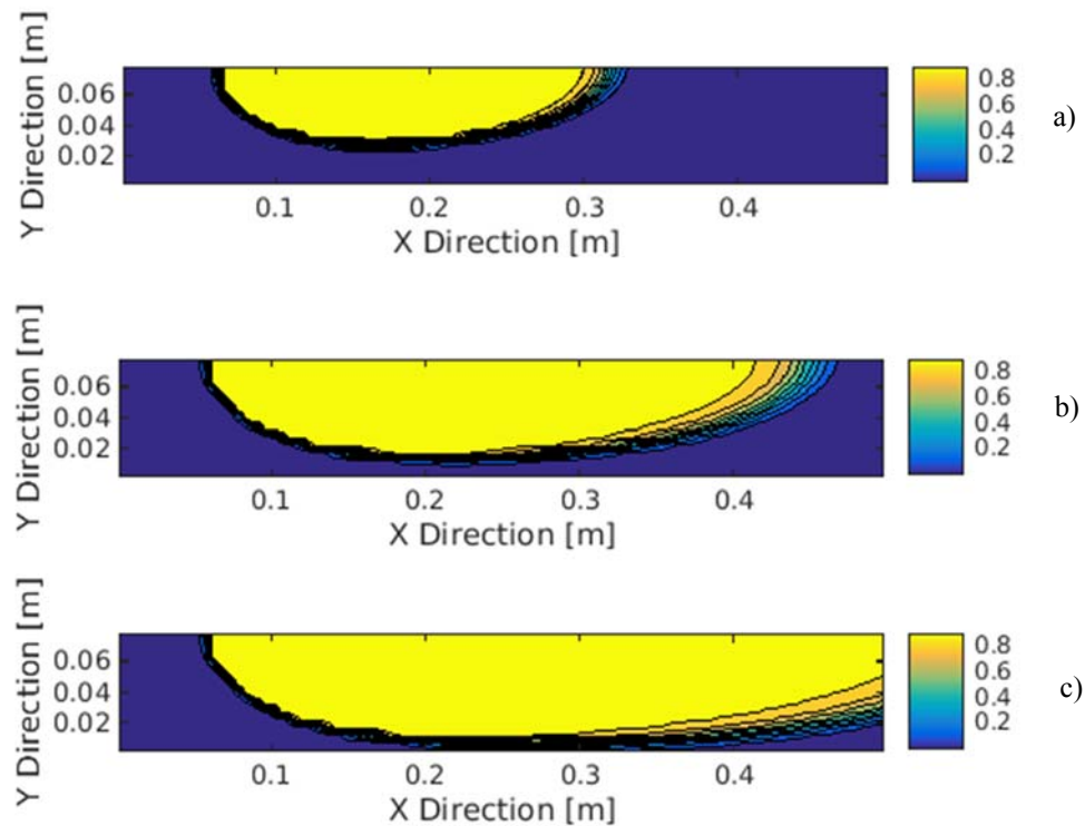
Figure 4: Saturation fields found by the numerical model after a) 25, b) 50, and c) 75 seconds, when using \beta = 1; L = -7.5; N = 4.5 .
