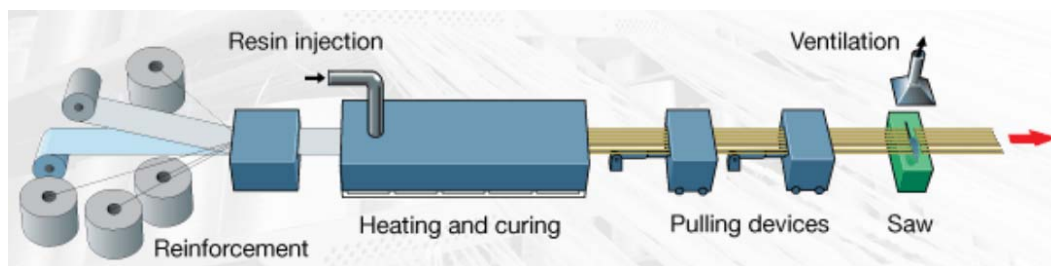
Figure 1: Sketch of the RIP process (courtesy of Fiberline).
