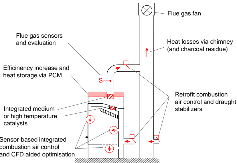
Figure 62: Overview on all system components regarded or optimized in the project. PCM : Phase Change Materials. CFD Computational Fluid Dynamics (source: TFZ)
