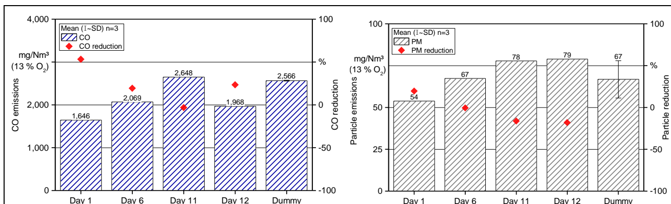
Figure 44: Long-term performance of the catalytic foam ceramic regarding CO emissions (left) and particle emissions (right)
