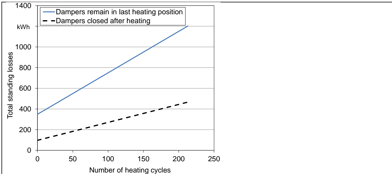
Figure 52: Aggregated total standing losses as a function of the number of annual heating cycles (calculated on measurement results for Stove A)
