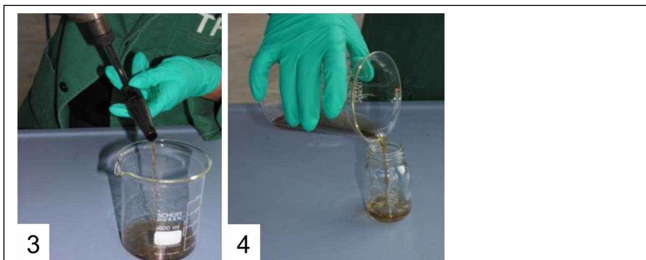
Figure 60: Execution of rinsing of PM sampling tract (source: TFZ)
