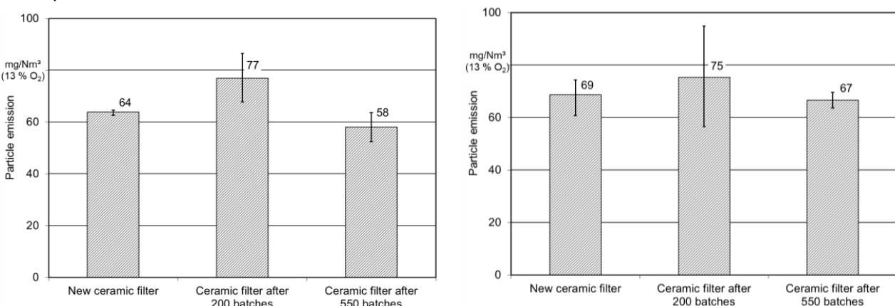
Figure 39: Particle emissions using three differently aged foam ceramic filters for full load operation (left) and part load operation (right)
