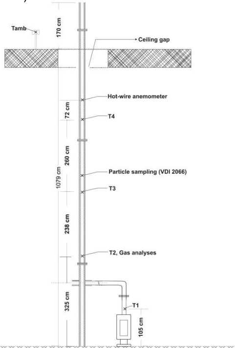
Figure 48: Dimensions of test rig and sensor positions in chimney
