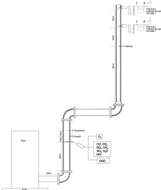
Figure 36: Test stand with flue gas tract for flue gas emission measurements
