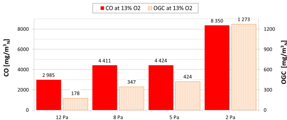
Figure 57: Comparison of CO & OGC for ignition batch at different draft levels
