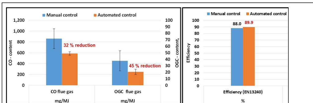
Figure 63: Emission reduction and efficiency increase achieved by implementing an automated control system in a newly developed low-emission stove (Source: BIOS)
