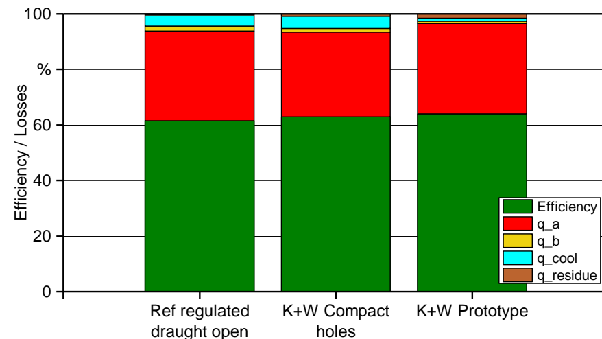
Figure 18: Comparison of auto adaptive (K+W prototype) and standard controller (K+W) in terms of efficiency.
