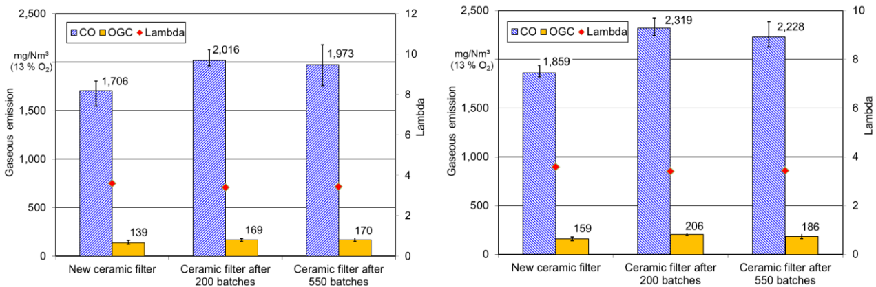
Figure 38: Gaseous emissions using three differently aged foam ceramic filters for full load operation (left) and part load operation (right)
