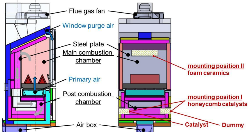
Figure 27: Schemes of the Low-emission wood stove used for catalyst testing
