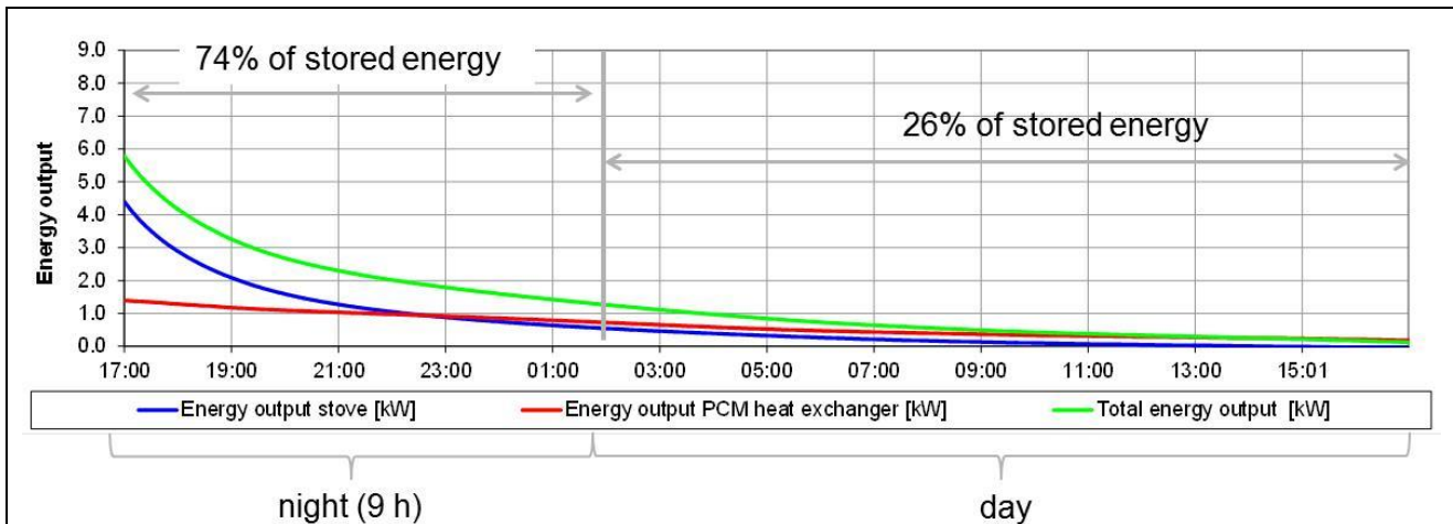
Figure 26: Unloading cycle of a wood stove with integrated heat storage unit based on PCM by natural convection
