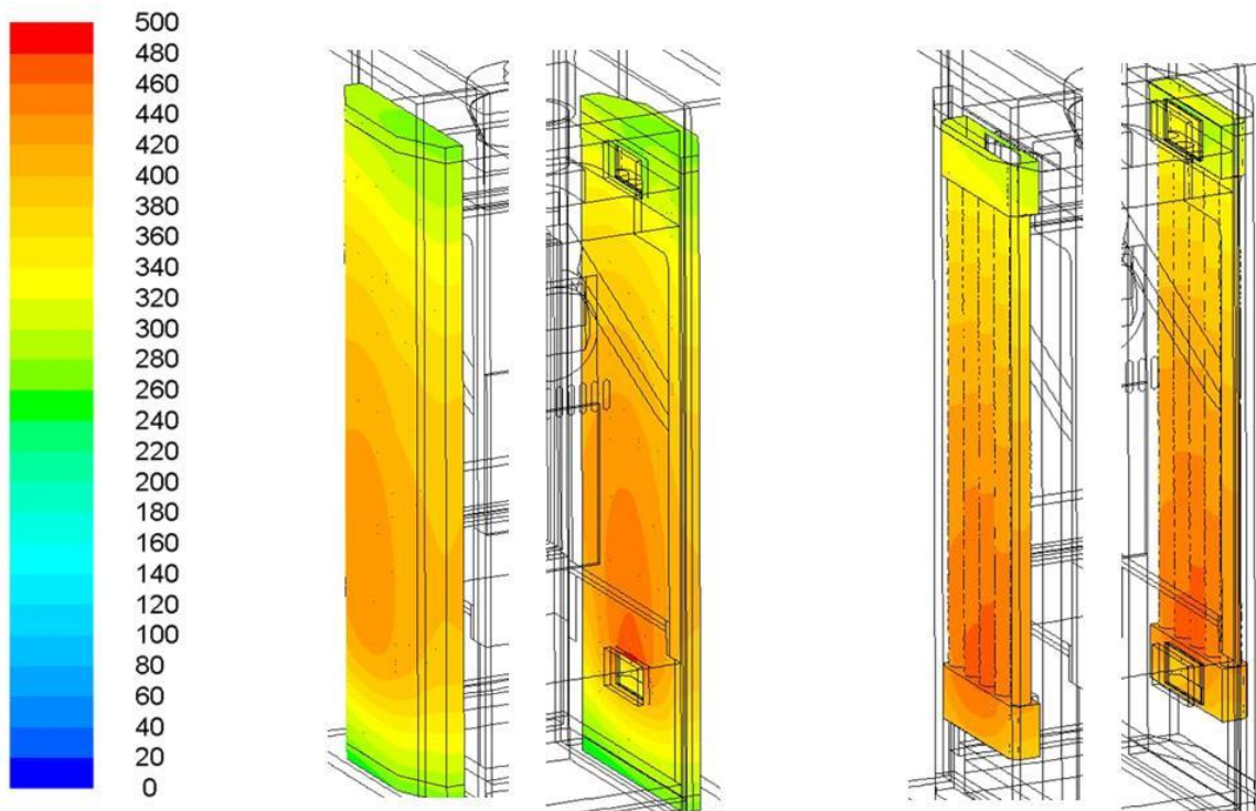
Figure 46: Iso-surfaces of material temperature [°C] in the PCM heat storage unit (steady state after complete charging); 3D view from the left and right hand side of the air channels
