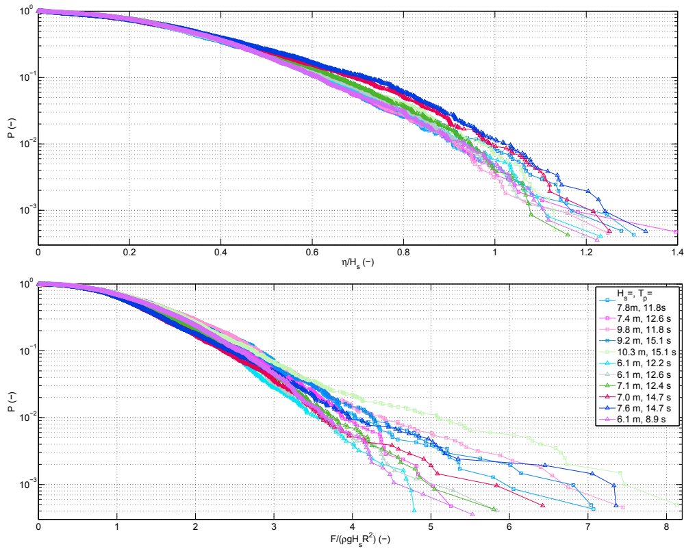
Fig. 3: Probability of exceedance of the crest heights and force peaks, when normalizing with H_s . \square h = 33\text{m} , \triangle h = 20\text{m} .
