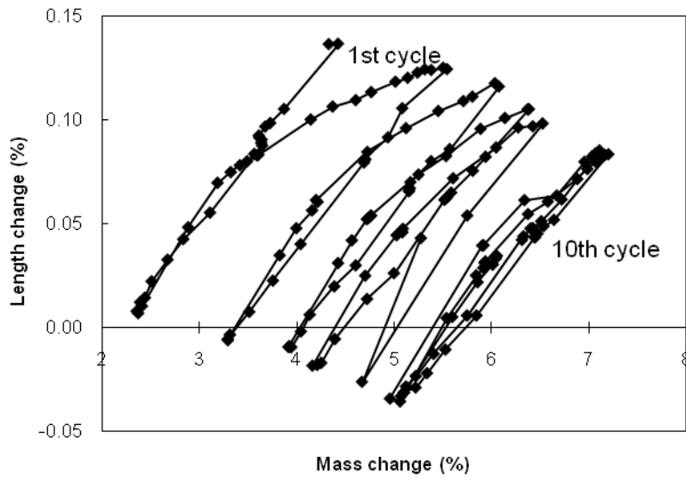
Figure 6 Plot of length against mass change of CBPB over series of cycles
