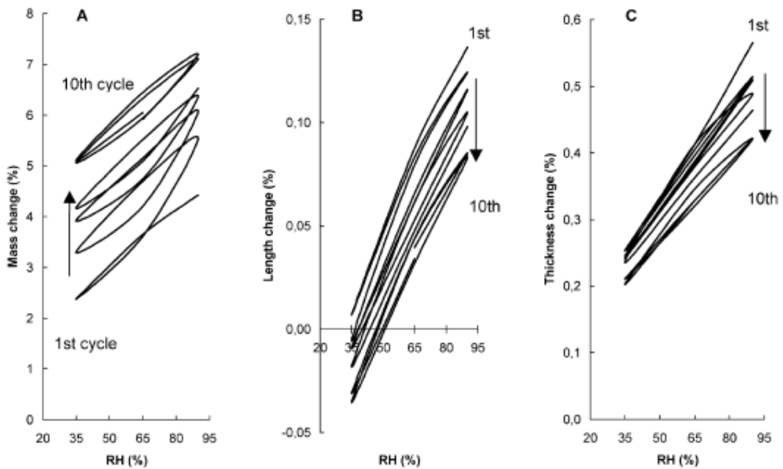
Figure 5 Sorption isotherms for mass (A), length (B) and thickness (C) of CBPB over a series of cycles
