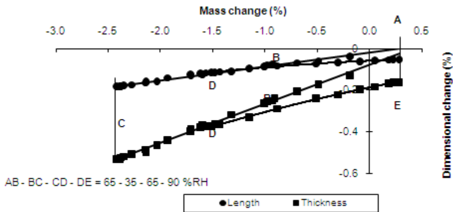
Figure 4 Experimental (markers) and calculated (lines) curves for CBPB in one complete cycle of cyclic RH
