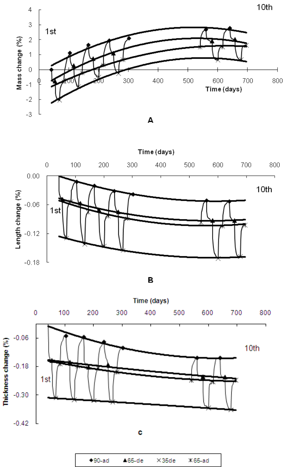
Figure 2 Experimentally determined and predicted change in mass (A), length (B) and thickness (C) of 12 mm CBPB (10 cycles in 90 - 65 - 35 - 65 - 90 %RH)
