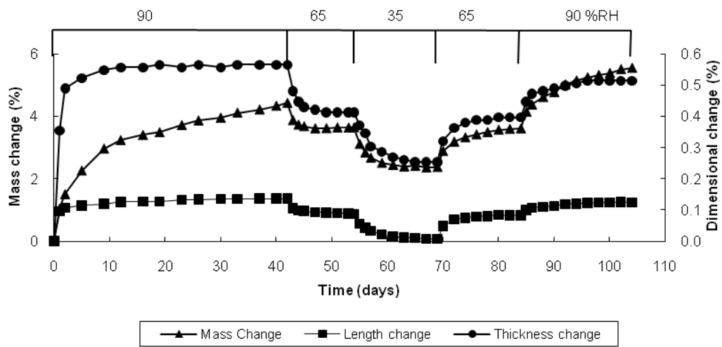
Figure 1 Change in mass and dimensions of CBPB over initial adsorption and the first complete cycle
