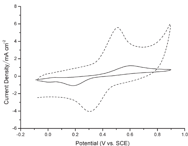
Fig. 3 – Cyclic voltammograms of dopamine ( 5 \cdot 10^{-3} M) at the bare platinum electrode (—) and the modified electrode (---). The background electrolyte is 0.1 M Na 2 SO 4 (pH ~ 6).
