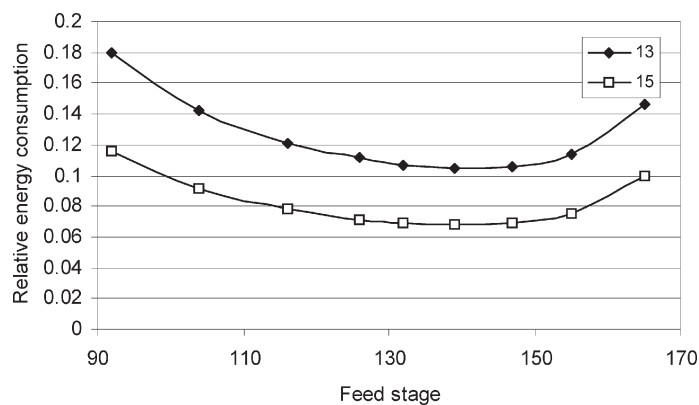
Fig. 8 – Relative energy consumption for HIDiC_upper with different feed stages compared to the conventional column
