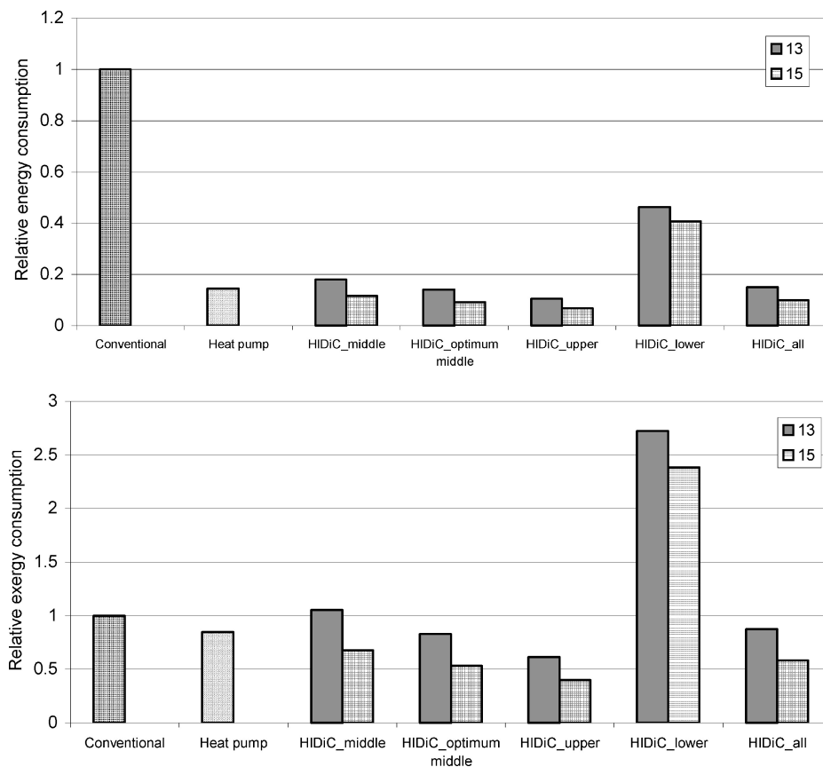
Fig. 3 – Relative energy (upper) and exergy (lower) consumption compared to the conventional column (HIDiC with bottom section pressure of respectively 13 and 15 bar)
