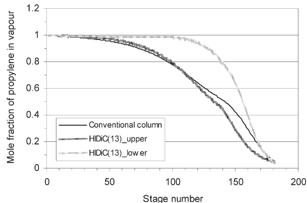
Fig. 5 – Comparison of propylene fraction in vapour along the conventional column, HIDiC_upper and HIDiC_lower
