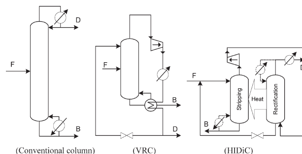
Fig. 1 – Schematic of the operating principle of a conventional column, a column with direct vapour recompression (VRC) and a HIDiC
