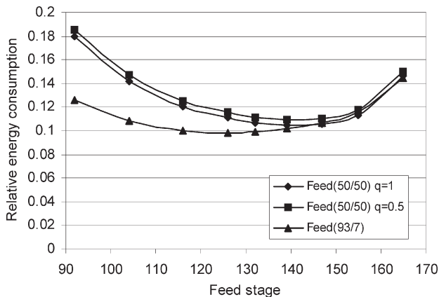
Fig. 9 – Effect of feed composition and feed thermal condition on the relative energy consumption of the HIDiC(13)_upper
