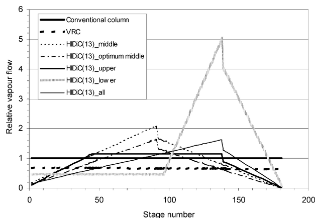
Fig. 4 – Comparison of vapour flow profiles for the high compression ratio HIDiC
