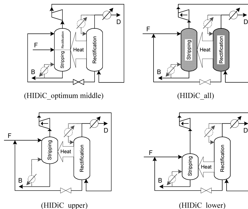
Fig. 2 – Other possible configurations of the HIDiC, in addition to that ( HIDiC_middle ) shown in Fig. 1
