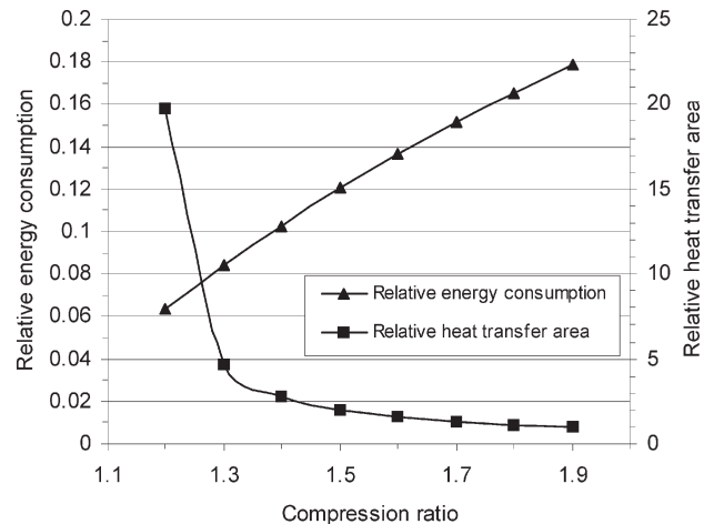
Fig. 10 – Effect of the compression ratio on the heat transfer area and the relative energy consumption of the HIDiC_upper
