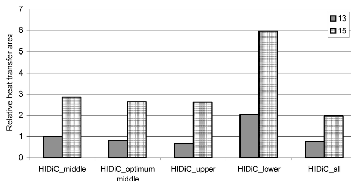
Fig. 6 – Heat transfer area relative to the HIDiC(15)_middle
