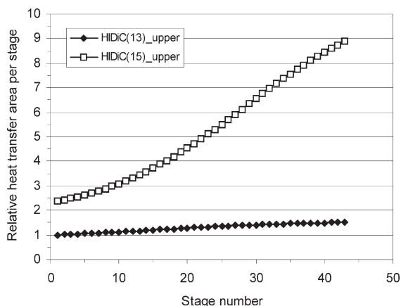
Fig. 7 – Effect of the compression ratio on the heat transfer area for HIDiC_upper
