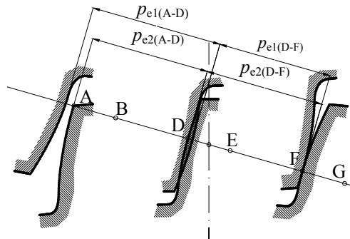
Slika 3h. Odstupanje koraka u trostrukom zahvatu, p_{e1(D-F)} > p_{e2(D-F)} , p_{e1(A-D)} + p_{e1(D-F)} < p_{e2(A-D)} + p_{e2(D-F)} Figure 3h. Pitch error in triple contact, p_{e1(D-F)} > p_{e2(D-F)} , p_{e1(A-D)} + p_{e1(D-F)} < p_{e2(A-D)} + p_{e2(D-F)}
