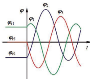
Slika 10 – Magnetski tokovi u jezgri trofaznog transformatora pri povoljno odabranom trenutku uklopa Figure 10 – Magnetic fluxes in the core of a three-phase transformer during optimal energization
