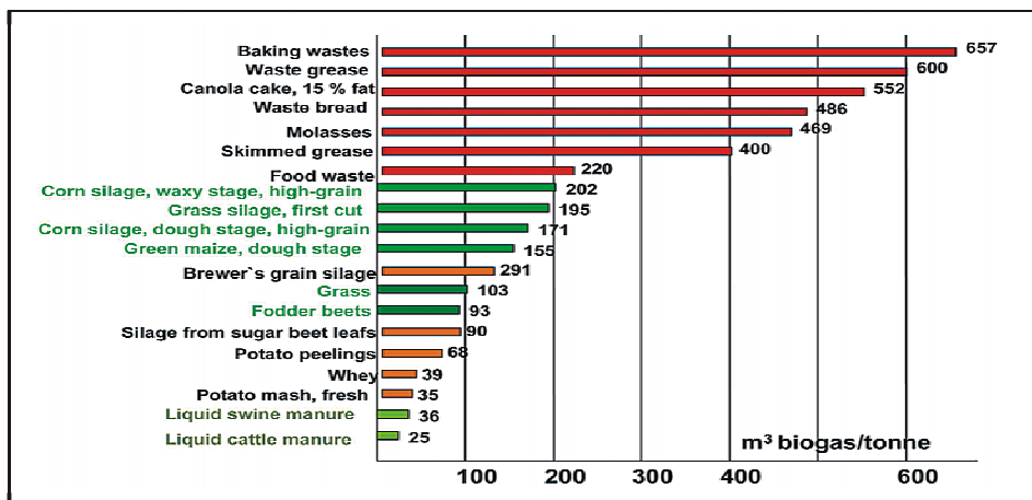
Fig.4. Potential biogas yields from different feedstock
