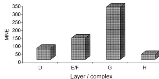
Fig. 5: Accumulated fossil remains of ungulata in taphodermes of layers/complexes D, E/F, G, and H.
