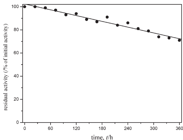
Fig. 5 – The stability of KcPGA at selected conditions of cefaclor synthesis Conditions: pH 6.5, 5 °C, 30 % ethylene glycol
