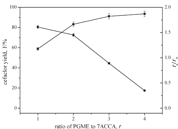
Fig. 4 – Effect of ratio of PGME to 7ACCA on the yield of cefaclor Reaction conditions: KcPGA 30 % ethylene glycol, 5 °C, 7ACCA 50 mmol L -1 , pH 6.5. Square: cefaclor yield; circle: r_s/r_h .
