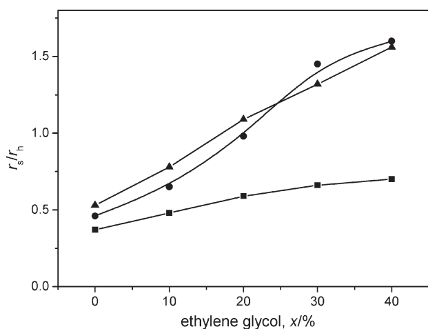
Fig. 2 – Effect of ethylene glycol fraction on the r_s/r_h of different immobilized penicillin acylase. Reaction conditions are the same as Fig. 1; Square: PCA; circle: KcPGA; uptriangle IPA750
