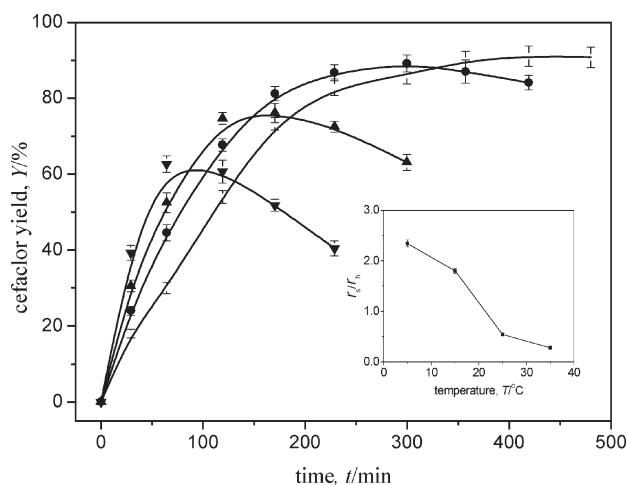
Fig. 3 – Effect of temperature on the yield of cefaclor in the presence of ethylene glycol. Reaction conditions: KcPGA, 30 % ethylene glycol, 50 mmol L -1 7ACCA, PGME 100 mmol L -1 , pH 6.5. Square: 5 °C; circle: 15 °C; uptriangle: 25 °C; downtriangle: 35 °C. r_s/r_h at different temperature was present at the inset.
