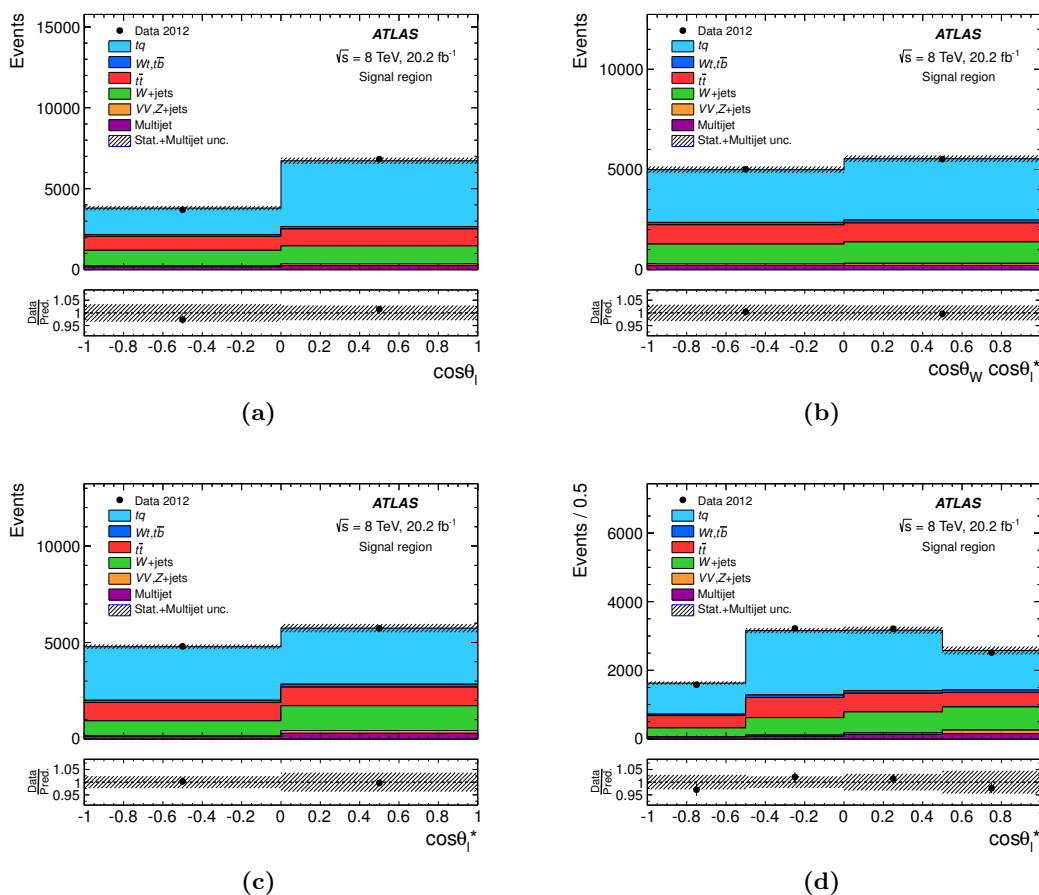
Figure 6. Distributions in the signal region of the angular observables used to measure the various asymmetries: (a) \cos\theta_\ell for A_{\text{FB}}^\ell , (b) \cos\theta_W \cos\theta_\ell^* for A_{\text{FB}}^W , (c) \cos\theta_\ell^* with two bins for A_{\text{FB}} , and (d) \cos\theta_\ell^* with four bins for A_{\text{EC}} . The observed distributions are compared to the predicted signal and background distributions, normalised to the results of the maximum-likelihood fit. The template t -channel distributions are taken from the baseline POWHEG-BOX sample. The labels tq and t\bar{b} refer to the t -channel and s -channel single-top-quark processes, respectively, and VV to diboson production. The uncertainty bands include the statistical post-fit uncertainty, the uncertainty due to the limited size of the simulation samples and the uncertainty in the normalisation of the multijet background, added in quadrature. The lower panels show the ratio of data to prediction.
