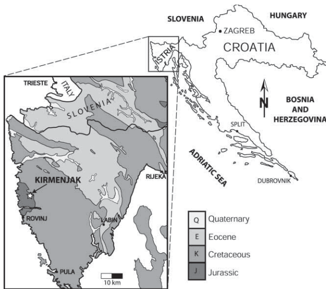
Figure 1: Geographic and geologic setting of the Kirmenjak locality in Istria, Croatia (modified after VELIĆ et al., 1995).
