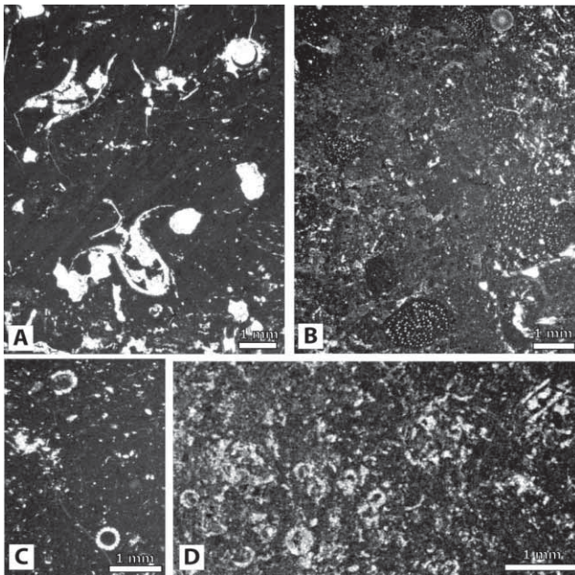
Figure 7: Microfossil assemblage of the Kirmenjak unit from the Kirmenjak quarry. A, longitudinal and transverse sections of Campbelliella striata (CAROZZI); B, fenestral mudstone with common Favreina sp.; C, algal mudstone with transverse sections of Salpingoporella annulata CAROZZI; and D, algal mudstone with various sections of S. annulata CAROZZI.
