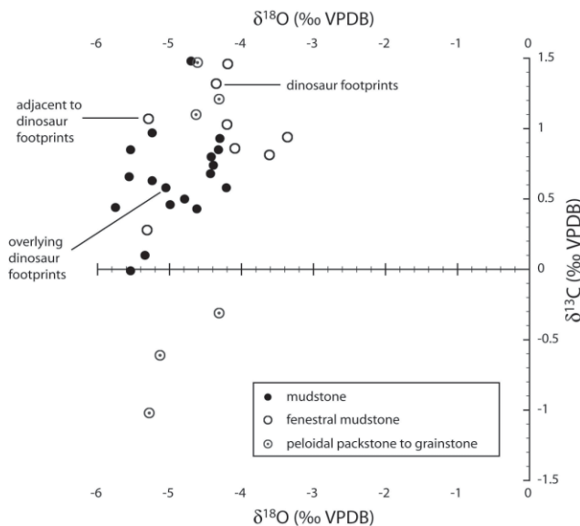
Figure 8: \delta^{13}\text{C} vs. \delta^{18}\text{O} values of the analyzed samples.
