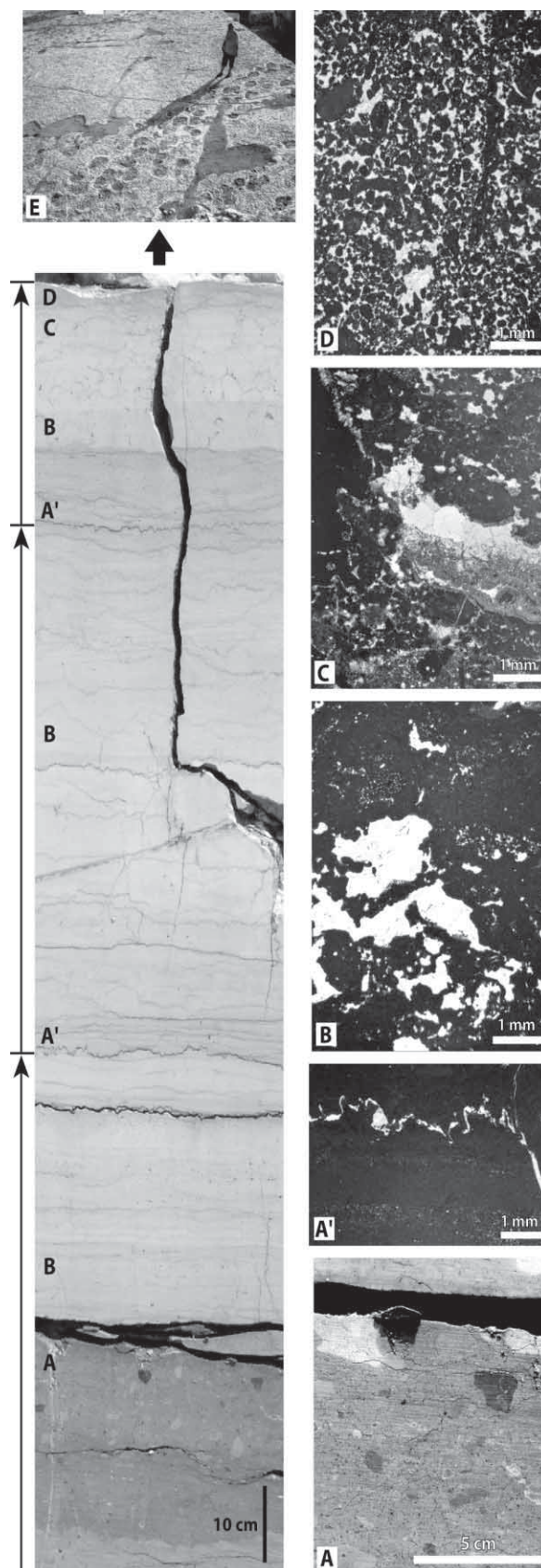
Figure 6: Details of shallowing upward cycles from the central part of the measured Kirmenjak succession (see also Fig. 2). The cycles begin with black pebble breccias (A) or stylolitized mudstone (A'), overlain by fenestral mudstone (B) and peloidal-intraclastic-fenestral packstone with geopetal infill (C), and capped with thin peloidal-intraclastic grainstone (D) with dinosaur footprints (E).
