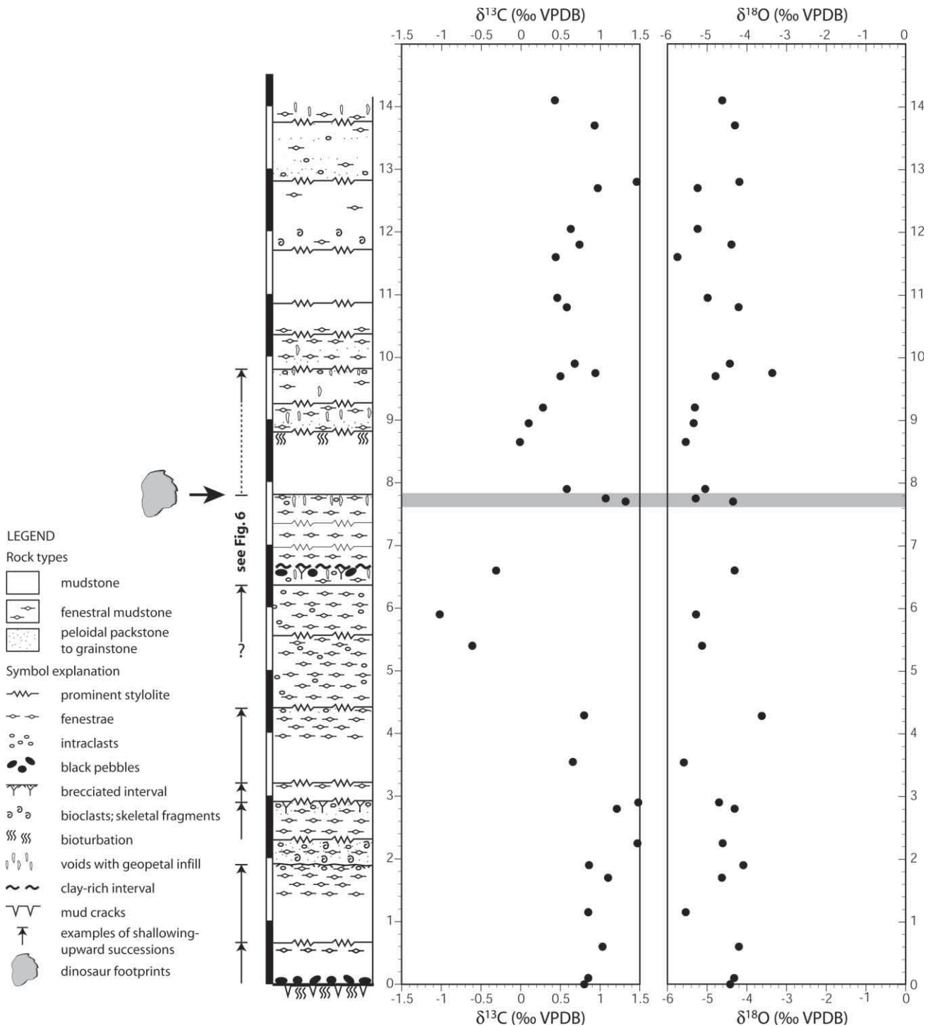
Figure 2: Schematic lithologic column of the measured Kirmenjak quarry succession with measured \delta^{13}\text{C} and \delta^{18}\text{O} values. Only examples of prominent shallowing-upward succession tops are indicated on the stratigraphic column.
