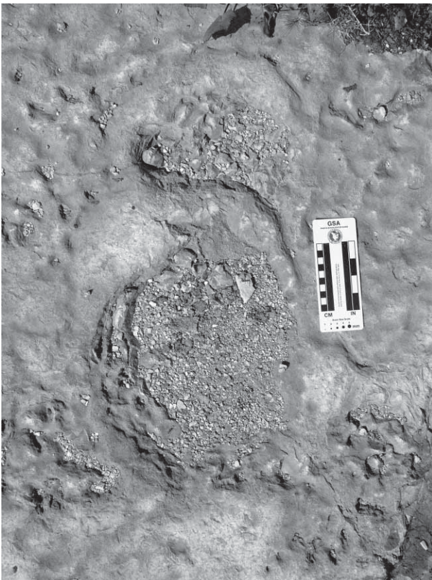
Figure 4: An oval-shaped pes print (lower part of the photograph) and a horseshoe-shaped manus print (upper part of the photograph) of the sauropod dinosaur from the Kirmenjajk quarry.
