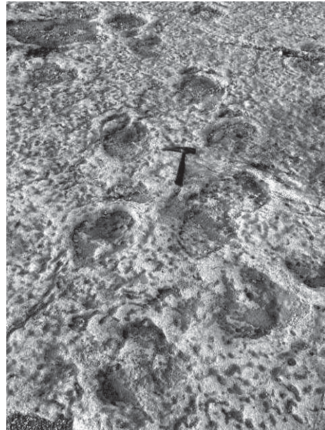
Figure 5: A narrow-gauge trackway of a sauropod dinosaur from the Kirmenjajk quarry.
