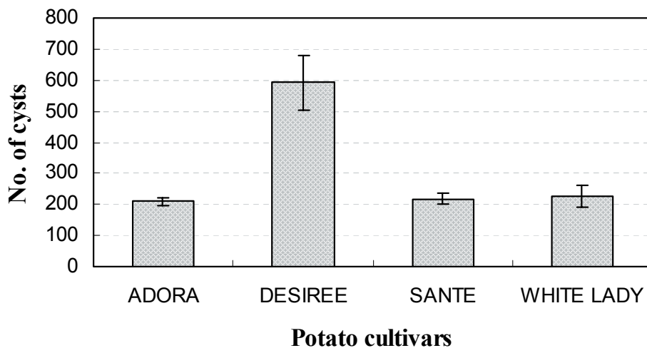
Graph 2: Total number of cysts of G. rostochiensis / 100 cm 3 soil sample (Pi = 208 ± 50)
