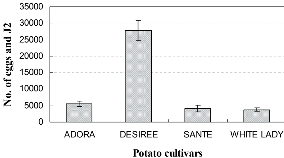
Graph 3: Total number of eggs and J2 of G. rostochiensis / 100 cm 3 soil sample ( P_i = 7013 \pm 2340 )
