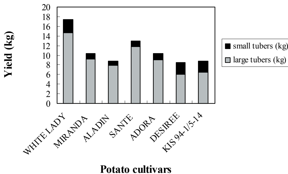
Graph 1: Potato yield in different potato cultivars
