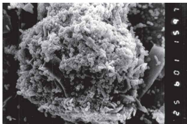
Fig. 2. White foam glass with the yeast after 2 h of shaking, magnification ×600. Figure is reproduced at 80 % of the original
