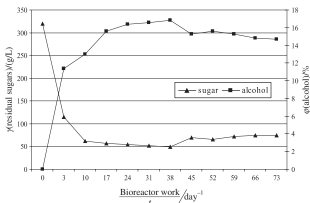
Fig. 1. Effect of fermentation time on alcohol fraction and residual sugars in fruit wine
