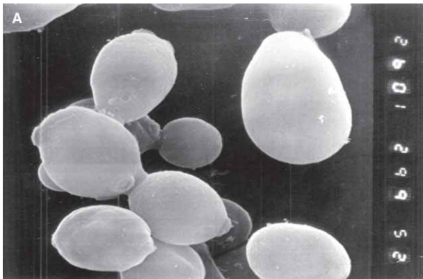
Fig. 5. Yeast cells isolated from the carrier from the first column, magnification \times 1200 . Figure is reproduced at 80 % of the original
