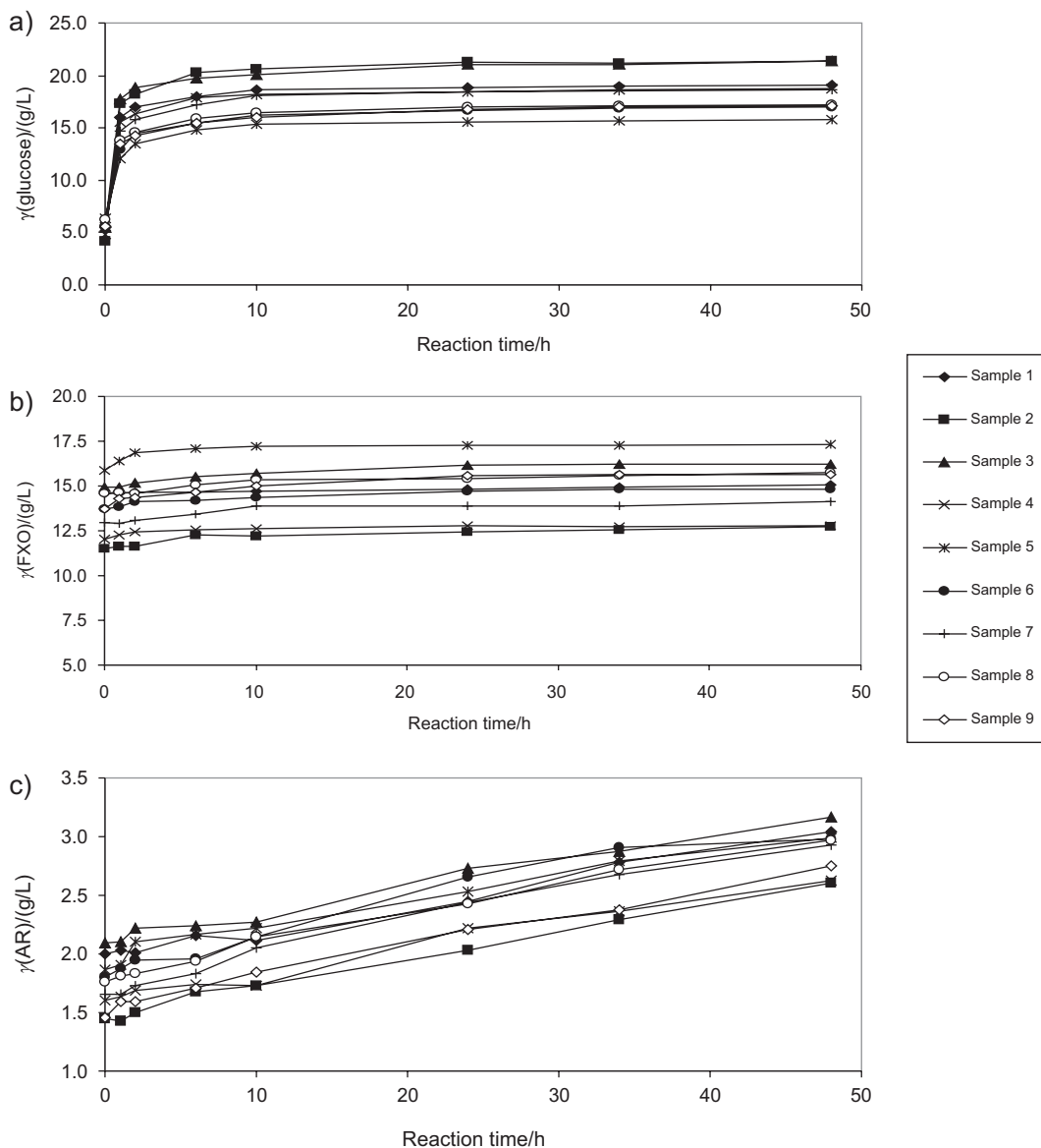
Fig. 2. Time course of sugars and malic acid concentration in enzymatic hydrolysates: a) glucose, b) fructose, xylose, mannose, galactose and malic acid, c) arabinose and rhamnose, N =2
