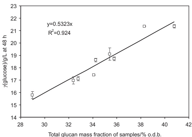
Fig. 3. Dependence of glucose concentration measured at 48 h in hydrolysates on total glucan mass fraction in samples, N =2
